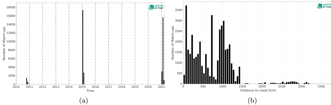
Figure 1: Number of match-ups between TSG (GOSUD-Research-vessel) and SMOS SSS L2Q v331 - No FLAG (CMEMS-CATDS-CPDC) SSS as a function of time (a) and as function of the distance to coast (b) over the Roaring Forties and Furious Fifties Pi-MEP region and for the full satellite product period.
