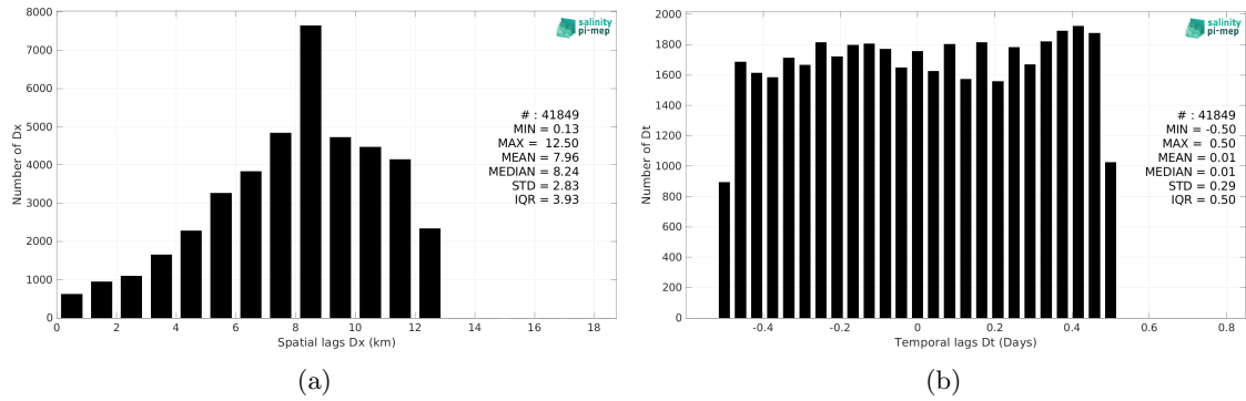
Figure 5: Histograms of the spatial (a) and temporal (b) lags between the location/time of the TSG (GOSUD-Research-vessel) measurement and the date of the corresponding SMOS SSS L2Q v331 - No FLAG (CMEMS-CATDS-CPDC) SSS pixel.
