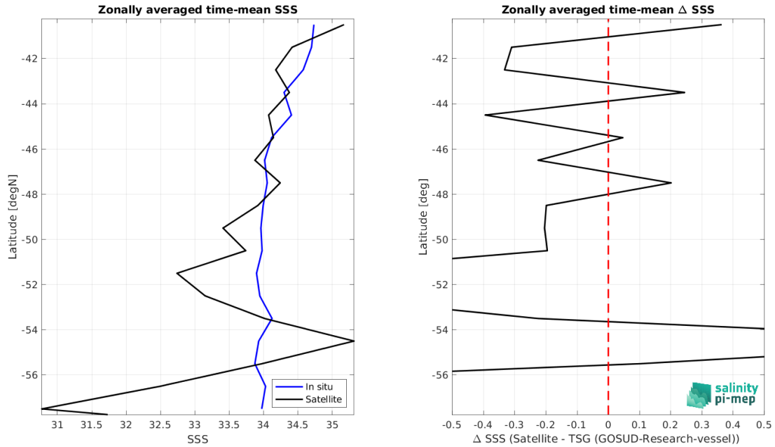
Figure 8: Left panel: Zonal mean SSS from SMOS SSS L2Q v331 - No FLAG (CMEMS-CATDS-CPDC) satellite product (black) and from TSG (GOSUD-Research-vessel) (blue). Right panel: Zonal mean of \Delta SSS (Satellite - TSG (GOSUD-Research-vessel)) for all the collected Pi-MEP match-up pairs estimated over the full satellite product period.
