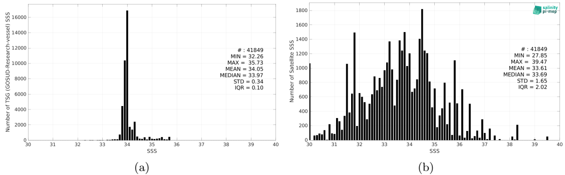
Figure 2: Histograms of SSS from TSG (GOSUD-Research-vessel) (a) and SMOS SSS L2Q v331 - No FLAG (CMEMS-CATDS-CPDC) (b) considering all match-up pairs per bins of 0.1 over the Roaring Forties and Furious Fifties Pi-MEP region and for the full satellite product period.
