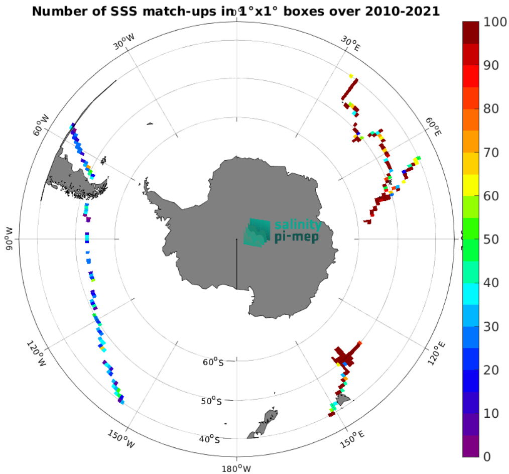
Figure 4: Number of SSS match-ups between TSG (GOSUD-Research-vessel) SSS and the SMOS SSS L2Q v331 - No FLAG (CMEMS-CATDS-CPDC) SSS product for the Roaring Forties and Furious Fifties Pi-MEP region over 1^\circ \times 1^\circ boxes and for the full satellite product period.
