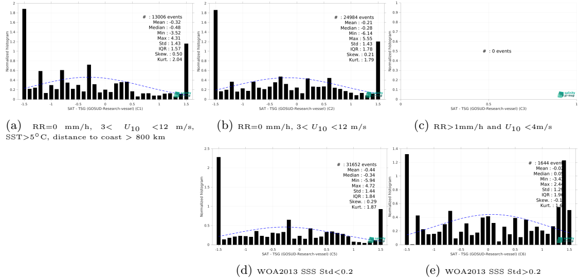
Figure 13: Normalized histogram of \Delta SSS (SMOS SSS L2Q v331 - No FLAG (CMEMS-CATDS-CPDC) - TSG (GOSUD-Research-vessel)) for 5 different subdatasets corresponding to: RR=0 mm/h, 3 < U_{10} < 12 m/s, SST > 5°C, distance to coast > 800 km (a), RR=0 mm/h, 3 < U_{10} < 12 m/s (b), RR > 1mm/h and U_{10} < 4 m/s (c), WOA2013 SSS Std < 0.2 (d), WOA2013 SSS Std > 0.2 (e).
