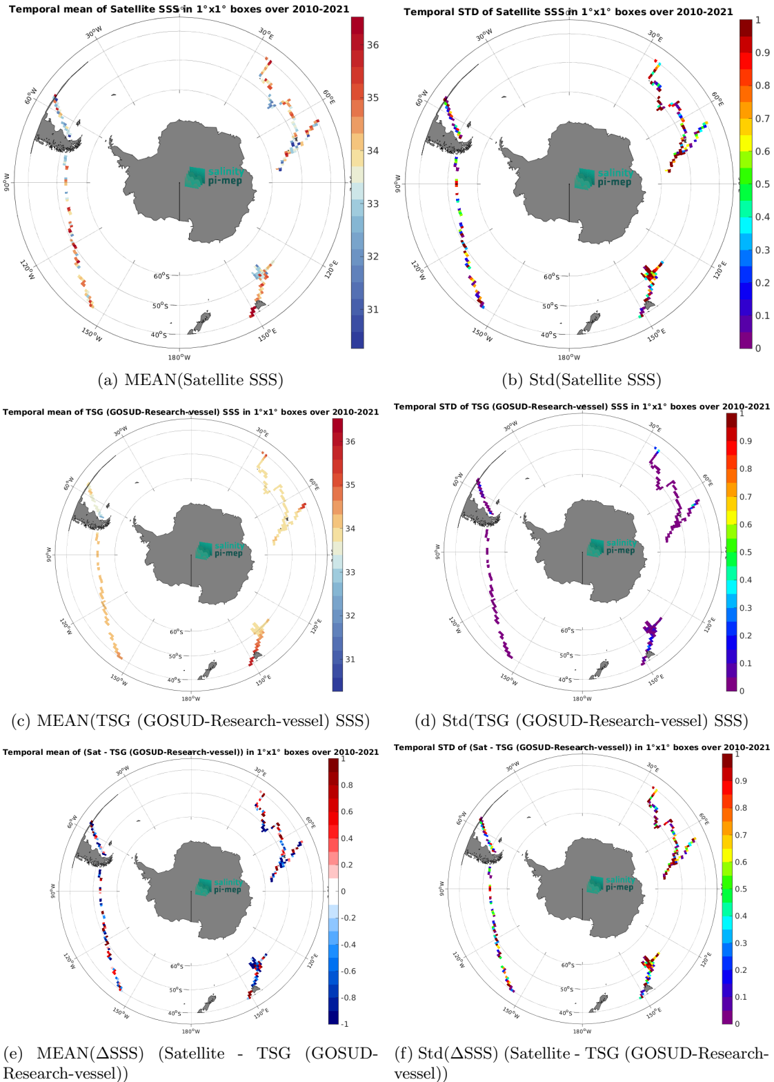
Figure 6: Temporal mean (left) and Std (right) of SSS from SMOS SSS L2Q v331 - No FLAG (CMEMS-CATDS-CPDC) (top), TSG (GOSUD-Research-vessel) (middle), and of \Delta SSS (Satellite - TSG (GOSUD-Research-vessel)). Only match-up pairs are used to generate these maps.
