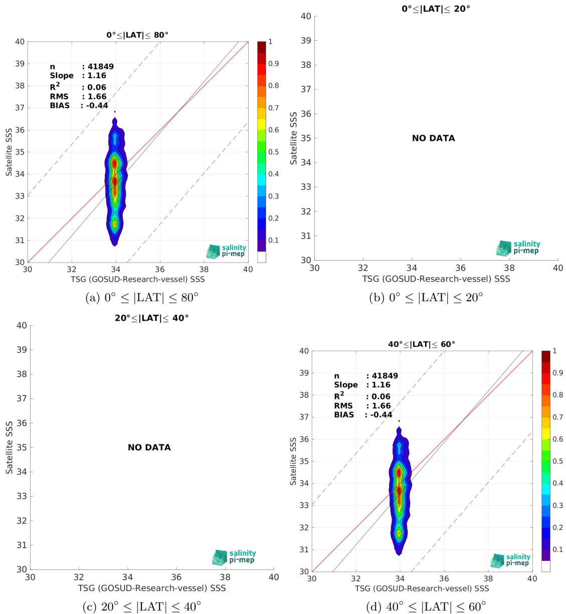
Figure 9: Contour maps of the concentration of SMOS SSS L2Q v331 - No FLAG (CMEMS-CATDS-CPDC) SSS (y-axis) versus TSG (GOSUD-Research-vessel) SSS (x-axis) at match-up pairs for different latitude bands. For each plot, the red line shows x=y . The black thin and dashed lines indicate a linear fit through the data cloud and the \pm 95\% confidence levels, respectively. The number match-up pairs n , the slope and R^2 coefficient of the linear fit, the root mean square (RMS) and the mean bias between satellite and in situ data are indicated for each latitude band in each plots.
