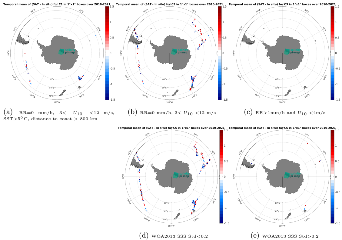
Figure 12: Temporal mean gridded over spatial boxes of size 1^\circ \times 1^\circ of \Delta\text{SSS} (SMOS SSS L2Q v331 - No FLAG (CMEMS-CATDS-CPDC) - TSG (GOSUD-Research-vessel)) for 5 different subdatasets corresponding to: RR=0 mm/h, 3 < U_{10} < 12 m/s, SST > 5^\circ\text{C} , distance to coast > 800 km (a), RR=0 mm/h, 3 < U_{10} < 12 m/s (b), RR > 1 mm/h and U_{10} < 4 m/s (c), WOA2013 SSS Std < 0.2 (d), WOA2013 SSS Std > 0.2 (e).
