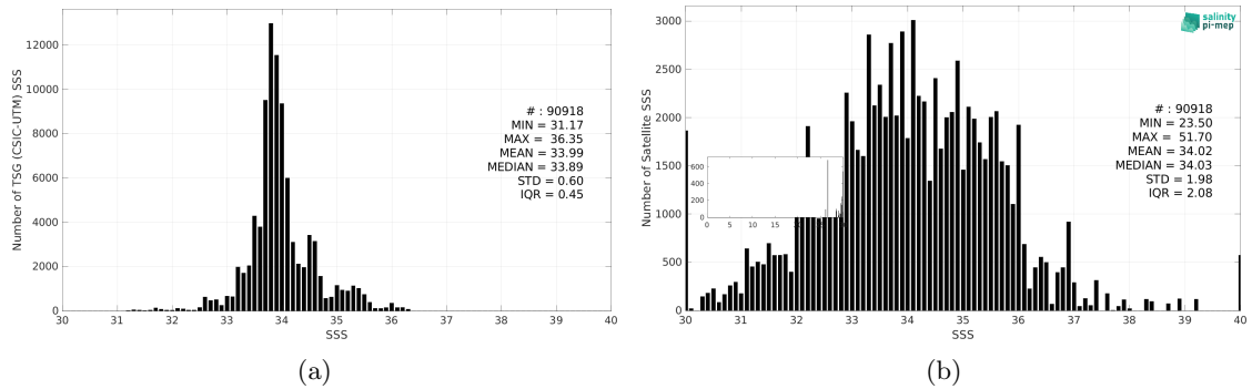
Figure 3: Histograms of SSS from TSG (CSIC-UTM) (a) and SMOS SSS L2Q v331 - No FLAG (CMEMS-CATDS-CPDC) (b) considering all match-up pairs per bins of 0.1 over the Roaring Forties and Furious Fifties Pi-MEP region and for the full satellite product period.
