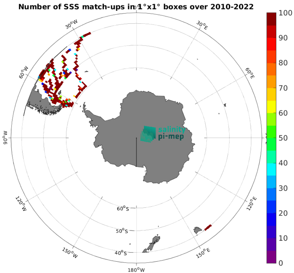
Figure 5: Number of SSS match-ups between TSG (CSIC-UTM) SSS and the SMOS SSS L2Q v331 - No FLAG (CMEMS-CATDS-CPDC) SSS product for the Roaring Forties and Furious Fifties Pi-MEP region over 1^{\circ} \times 1^{\circ} boxes and for the full satellite product period.
