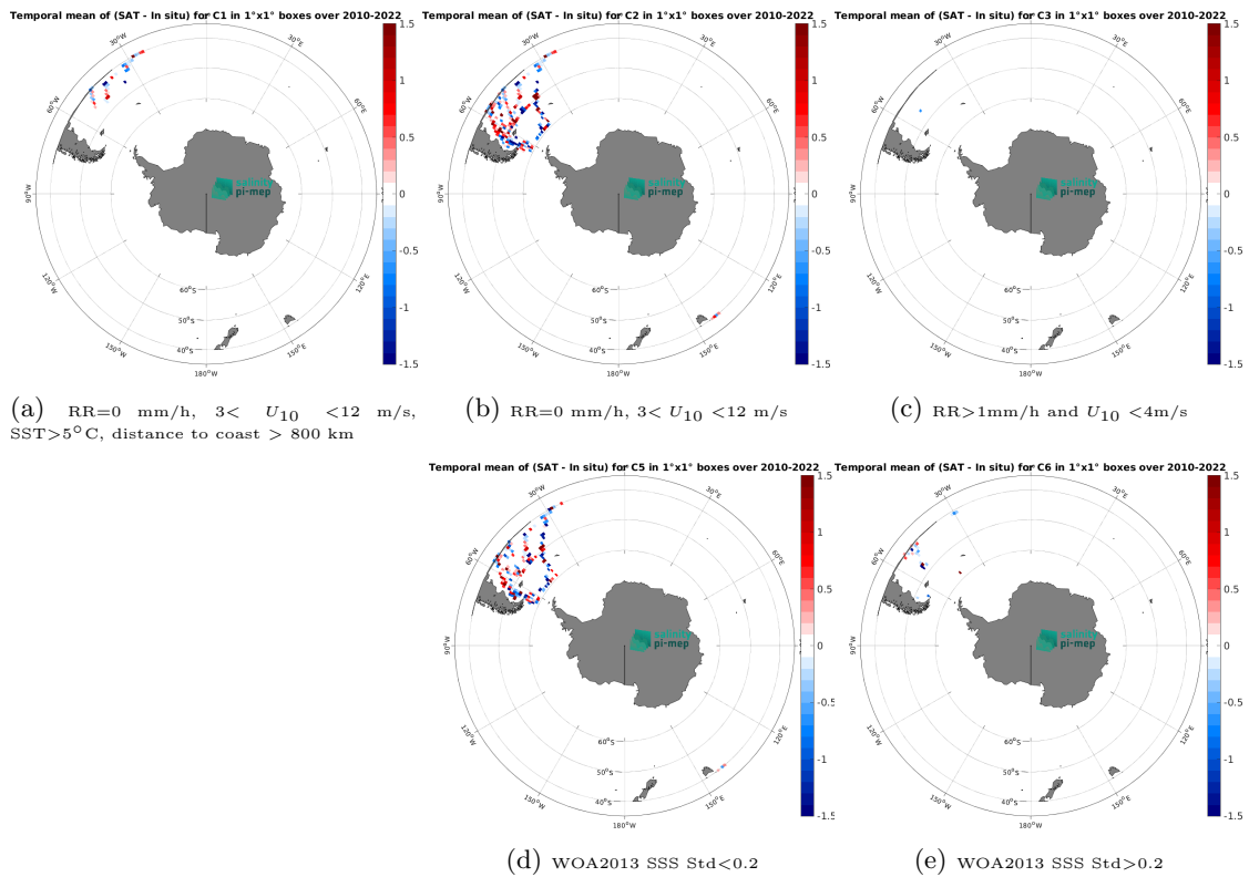
Figure 14: Temporal mean gridded over spatial boxes of size 1^\circ \times 1^\circ of \Delta SSS (SMOS SSS L2Q v331 - No FLAG (CMEMS-CATDS-CPDC) - TSG (CSIC-UTM)) for 5 different subdatasets corresponding to:RR=0 mm/h, 3 < U_{10} < 12 m/s, SST>5°C, distance to coast > 800 km (a), RR=0 mm/h, 3 < U_{10} < 12 m/s (b), RR>1mm/h and U_{10} < 4 m/s (c), WOA2013 SSS Std<0.2 (d), WOA2013 SSS Std>0.2 (e).
