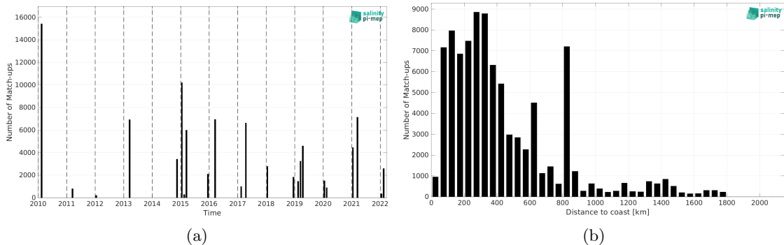
Figure 2: Number of match-ups between TSG (CSIC-UTM) and SMOS SSS L2Q v331 - No FLAG (CMEMS-CATDS-CPDC) SSS as a function of time (a) and as function of the distance to coast (b) over the Roaring Forties and Furious Fifties Pi-MEP region and for the full satellite product period.
