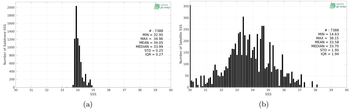
Figure 2: Histograms of SSS from Saildrone (a) and SMOS SSS L2Q v331 - No FLAG (CMEMS-CATDS-CPDC) (b) considering all match-up pairs per bins of 0.1 over the Roaring Forties and Furious Fifties Pi-MEP region and for the full satellite product period.
