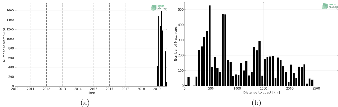
Figure 1: Number of match-ups between Saildrone and SMOS SSS L2Q v331 - No FLAG (CMEMS-CATDS-CPDC) SSS as a function of time (a) and as function of the distance to coast (b) over the Roaring Forties and Furious Fifties Pi-MEP region and for the full satellite product period.
