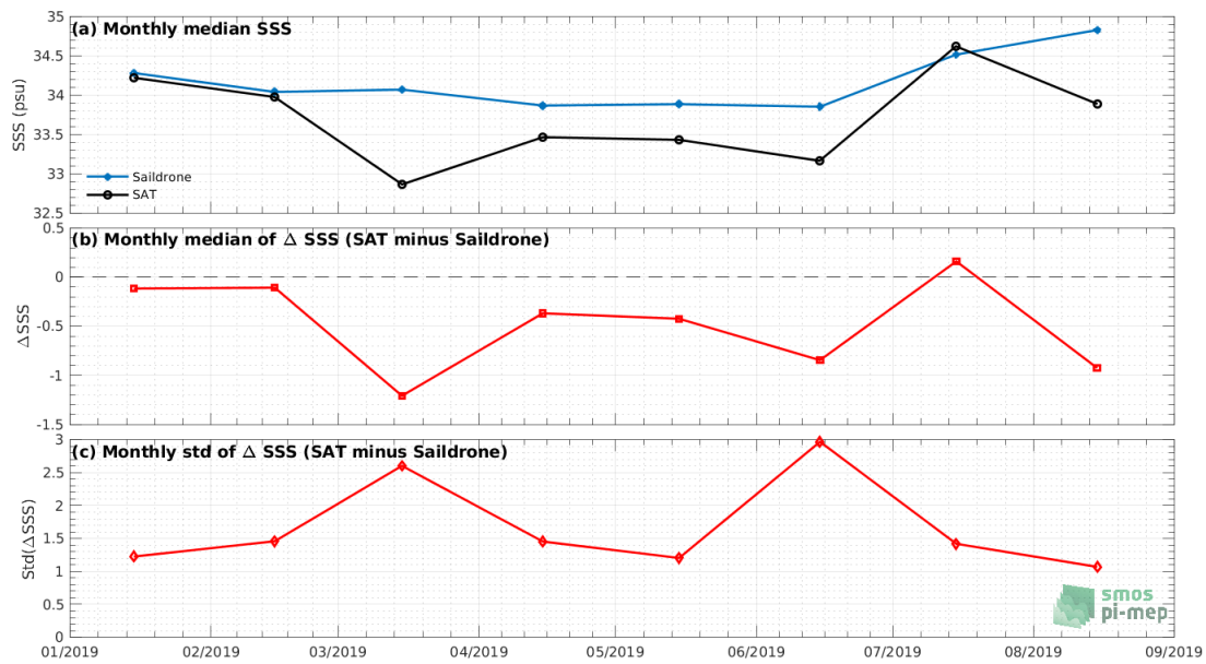
Figure 7: Time series of the monthly median SSS (top), median of \Delta SSS (Satellite - Sairdrone) and Std of \Delta SSS (Satellite - Sairdrone) over the Roaring Forties and Furious Fifties Pi-MEP region considering all match-ups collected by the Pi-MEP.
