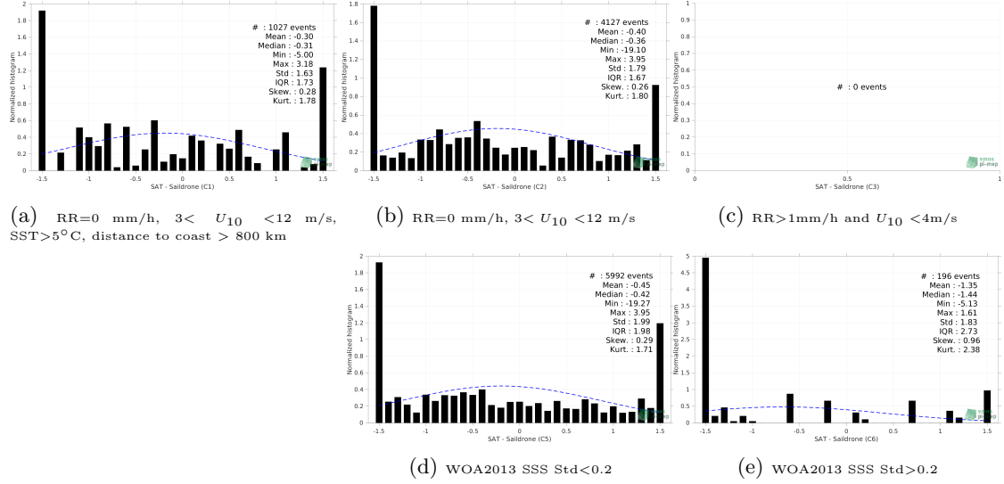
Figure 13: Normalized histogram of \Delta SSS (SMOS SSS L2Q v331 - No FLAG (CMEMS-CATDS-CPDC) - Saildrone) for 5 different subdatasets corresponding to: RR=0 mm/h, 3 < U_{10} < 12 m/s, SST > 5°C, distance to coast > 800 km (a), RR=0 mm/h, 3 < U_{10} < 12 m/s (b), RR > 1mm/h and U_{10} < 4 m/s (c), WOA2013 SSS Std < 0.2 (d), WOA2013 SSS Std > 0.2 (e).
