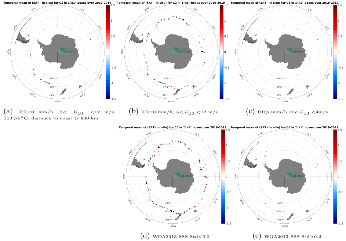
Figure 12: Temporal mean gridded over spatial boxes of size 1^{\circ}\times 1^{\circ} of \Delta\text{SSS} (SMOS SSS L2Q v331 - No FLAG (CMEMS-CATDS-CPDC) - Sairdrone) for 5 different subdatasets corresponding to:RR=0 mm/h, 3 < U_{10} < 12 m/s, SST > 5^{\circ}\text{C} , distance to coast > 800 km (a), RR=0 mm/h, 3 < U_{10} < 12 m/s (b), RR > 1 mm/h and U_{10} < 4 m/s (c), WOA2013 SSS Std < 0.2 (d), WOA2013 SSS Std > 0.2 (e).
