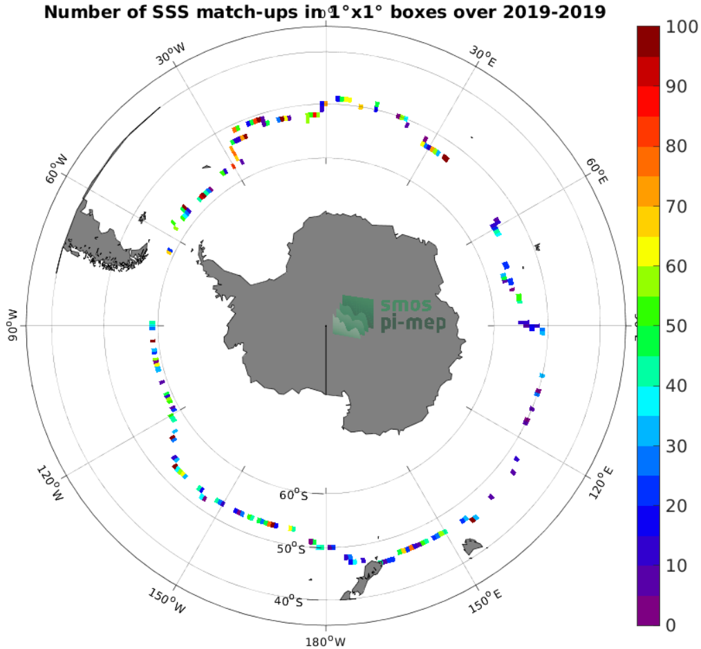
Figure 4: Number of SSS match-ups between Saildrone SSS and the SMOS SSS L2Q v331 - No FLAG (CMEMS-CATDS-CPDC) SSS product for the Roaring Forties and Furious Fifties Pi-MEP region over 1^\circ \times 1^\circ boxes and for the full satellite product period.
