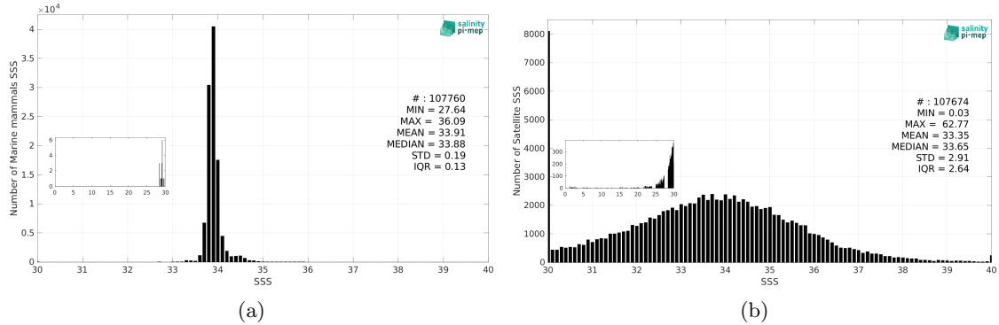
Figure 3: Histograms of SSS from Marine mammals (a) and SMOS SSS L2Q v331 - No FLAG (CMEMS-CATDS-CPDC) (b) considering all match-up pairs per bins of 0.1 over the Roaring Forties and Furious Fifties Pi-MEP region and for the full satellite product period.
