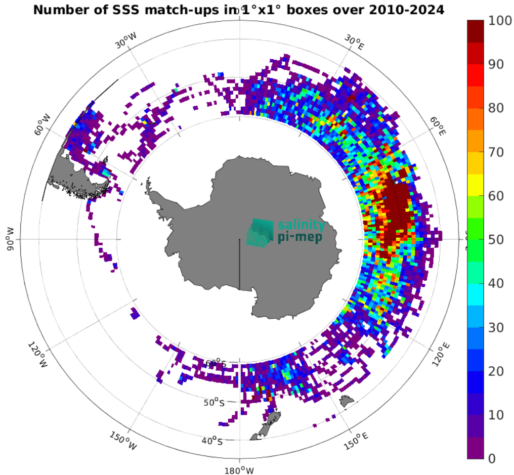
Figure 5: Number of SSS match-ups between Marine mammals SSS and the SMOS SSS L2Q v331 - No FLAG (CMEMS-CATDS-CPDC) SSS product for the Roaring Forties and Furious Fifties Pi-MEP region over 1^\circ \times 1^\circ boxes and for the full satellite product period.
