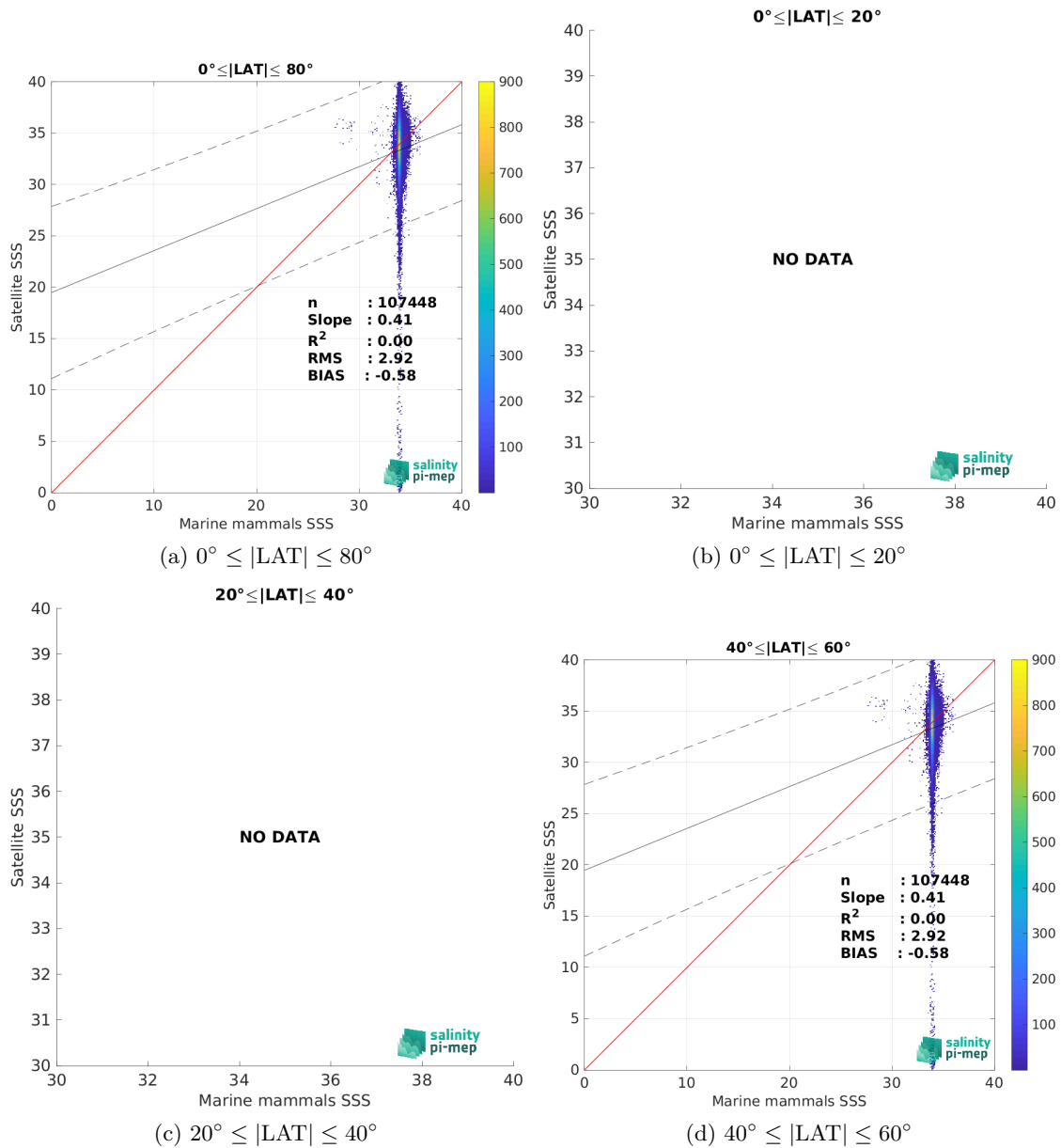
Figure 10: Contour maps of the concentration of SMOS SSS L2Q v331 - No FLAG (CMEMS-CATDS-CPDC) SSS (y-axis) versus Marine mammals SSS (x-axis) at match-up pairs for different latitude bands. For each plot, the red line shows x=y . The black thin and dashed lines indicate a linear fit through the data cloud and the \pm 95\% confidence levels, respectively. The number match-up pairs n , the slope and R^2 coefficient of the linear fit, the root mean square (RMS) and the mean bias between satellite and in situ data are indicated for each latitude band in each plots.
