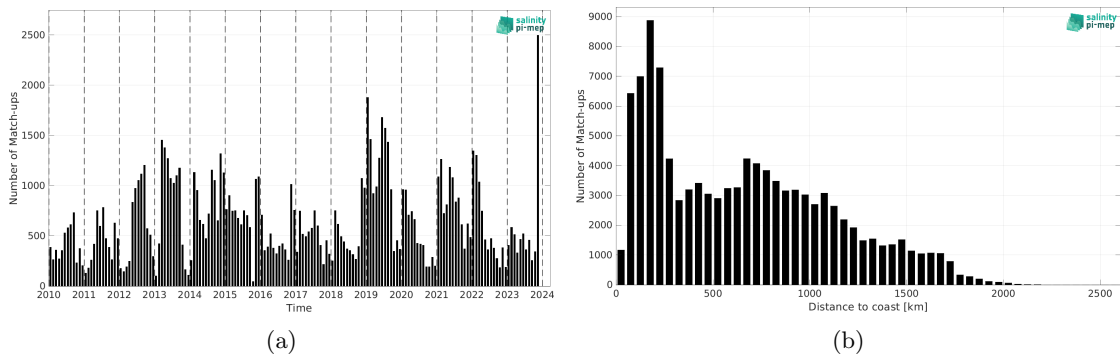
Figure 2: Number of match-ups between Marine mammals and SMOS SSS L2Q v331 - No FLAG (CMEMS-CATDS-CPDC) SSS as a function of time (a) and as function of the distance to coast (b) over the Roaring Forties and Furious Fifties Pi-MEP region and for the full satellite product period.
