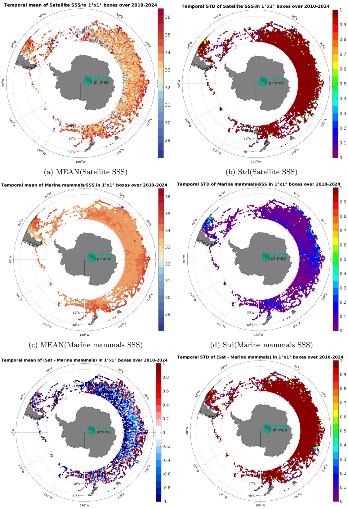
Figure 7: Temporal mean (left) and Std (right) of SSS from SMOS SSS L2Q v331 - No FLAG (CMEMS-CATDS-CPDC) (top), Marine mammals (middle), and of \Delta SSS (Satellite - Marine mammals). Only match-up pairs are used to generate these maps.
