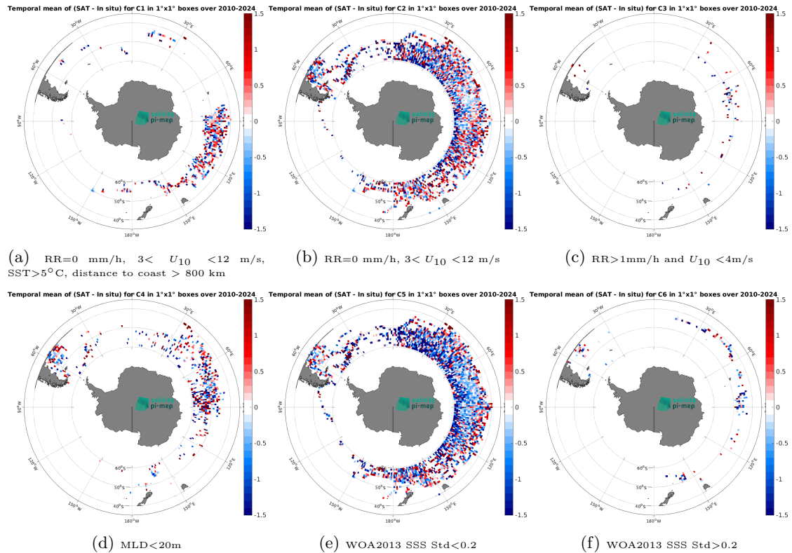
Figure 14: Temporal mean gridded over spatial boxes of size 1^\circ \times 1^\circ of \Delta\text{SSS} (SMOS SSS L2Q v331 - No FLAG (CMEMS-CATDS-CPDC) - Marine mammals) for 6 different subdatasets corresponding to:RR=0 mm/h, 3 < U_{10} < 12 m/s, SST>5°C, distance to coast > 800 km (a), RR=0 mm/h, 3 < U_{10} < 12 m/s (b), RR>1mm/h and U_{10} < 4 m/s (c),MLD<20m (d),WOA2013 SSS Std<0.2 (e),WOA2013 SSS Std>0.2 (f).
