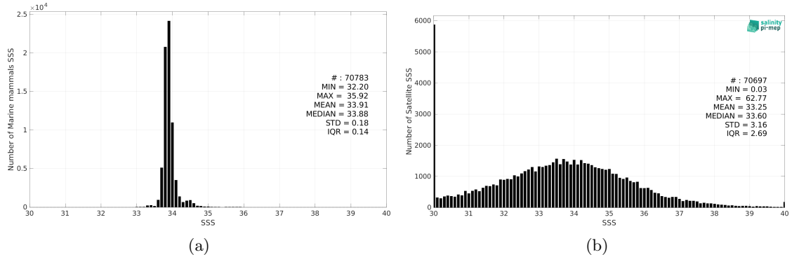
Figure 2: Histograms of SSS from Marine mammals (a) and SMOS SSS L2Q v331 - No FLAG (CMEMS-CATDS-CPDC) (b) considering all match-up pairs per bins of 0.1 over the Roaring Forties and Furious Fifties Pi-MEP region and for the full satellite product period.
