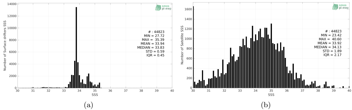
Figure 2: Histograms of SSS from Surface drifters (a) and SMOS SSS L2Q v331 - No FLAG (CMEMS-CATDS-CPDC) (b) considering all match-up pairs per bins of 0.1 over the Roaring Forties and Furious Fifties Pi-MEP region and for the full satellite product period.
