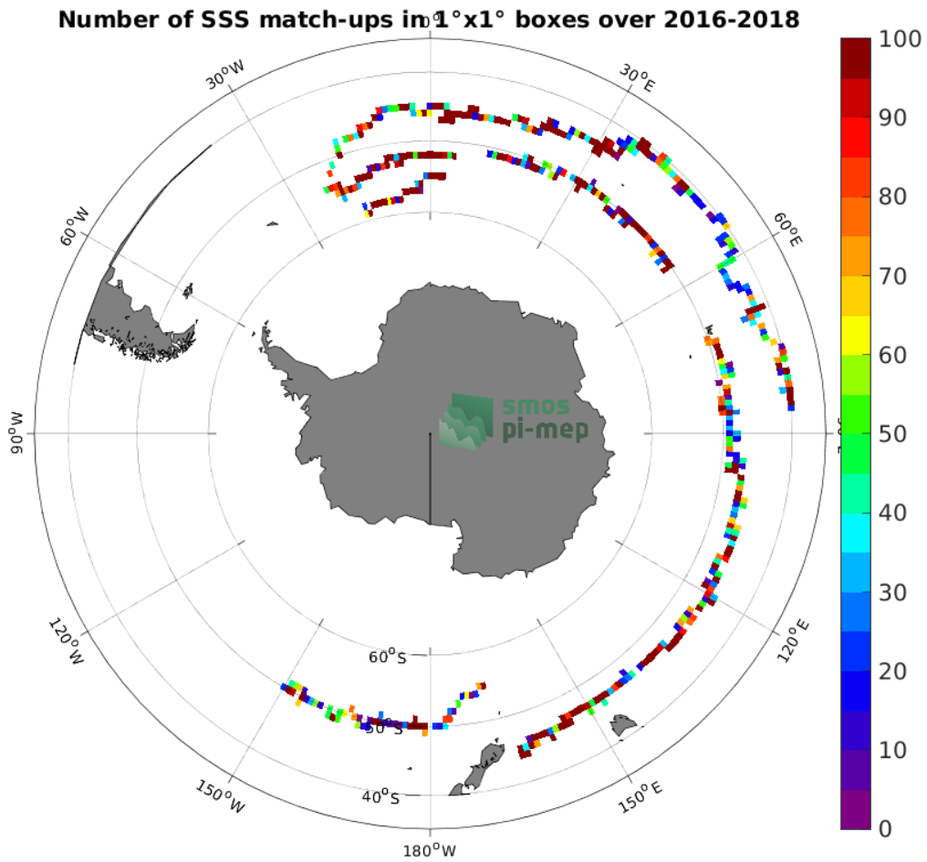
Figure 3: Number of SSS match-ups between Surface drifters SSS and the SMOS SSS L2Q v331 - No FLAG (CMEMS-CATDS-CPDC) SSS product for the Roaring Forties and Furious Fifties Pi-MEP region over 1^\circ \times 1^\circ boxes and for the full satellite product period.
