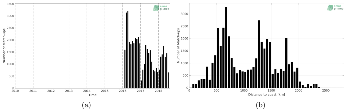
Figure 1: Number of match-ups between Surface drifters and SMOS SSS L2Q v331 - No FLAG (CMEMS-CATDS-CPDC) SSS as a function of time (a) and as function of the distance to coast (b) over the Roaring Forties and Furious Fifties Pi-MEP region and for the full satellite product period.
