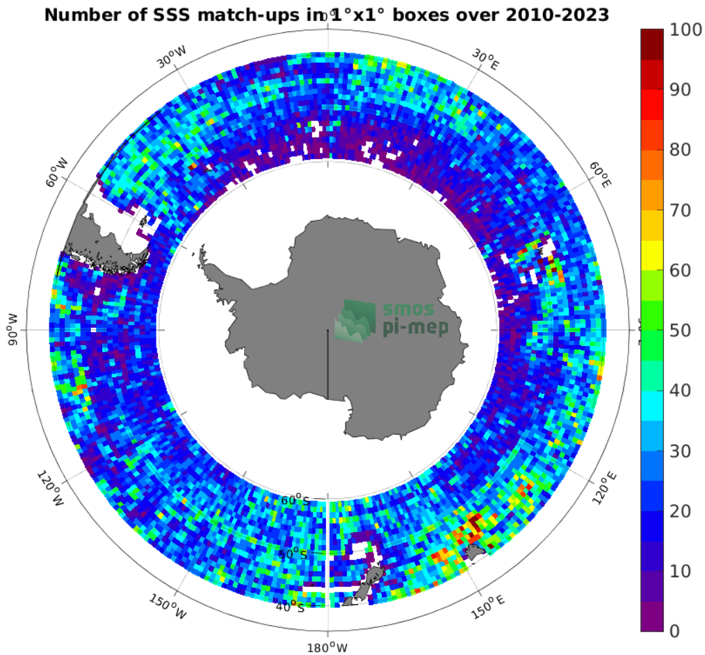
Figure 4: Number of SSS match-ups between Argo SSS and the SMOS SSS L2Q v331 - No FLAG (CMEMS-CATDS-CPDC) SSS product for the Roaring Forties and Furious Fifties Pi-MEP region over 1^\circ \times 1^\circ boxes and for the full satellite product period.
