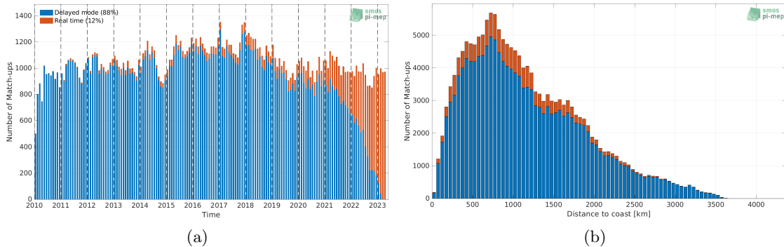
Figure 1: Number of match-ups between Argo and SMOS SSS L2Q v331 - No FLAG (CMEMS-CATDS-CPDC) SSS as a function of time (a) and as function of the distance to coast (b) over the Roaring Forties and Furious Fifties Pi-MEP region and for the full satellite product period.
