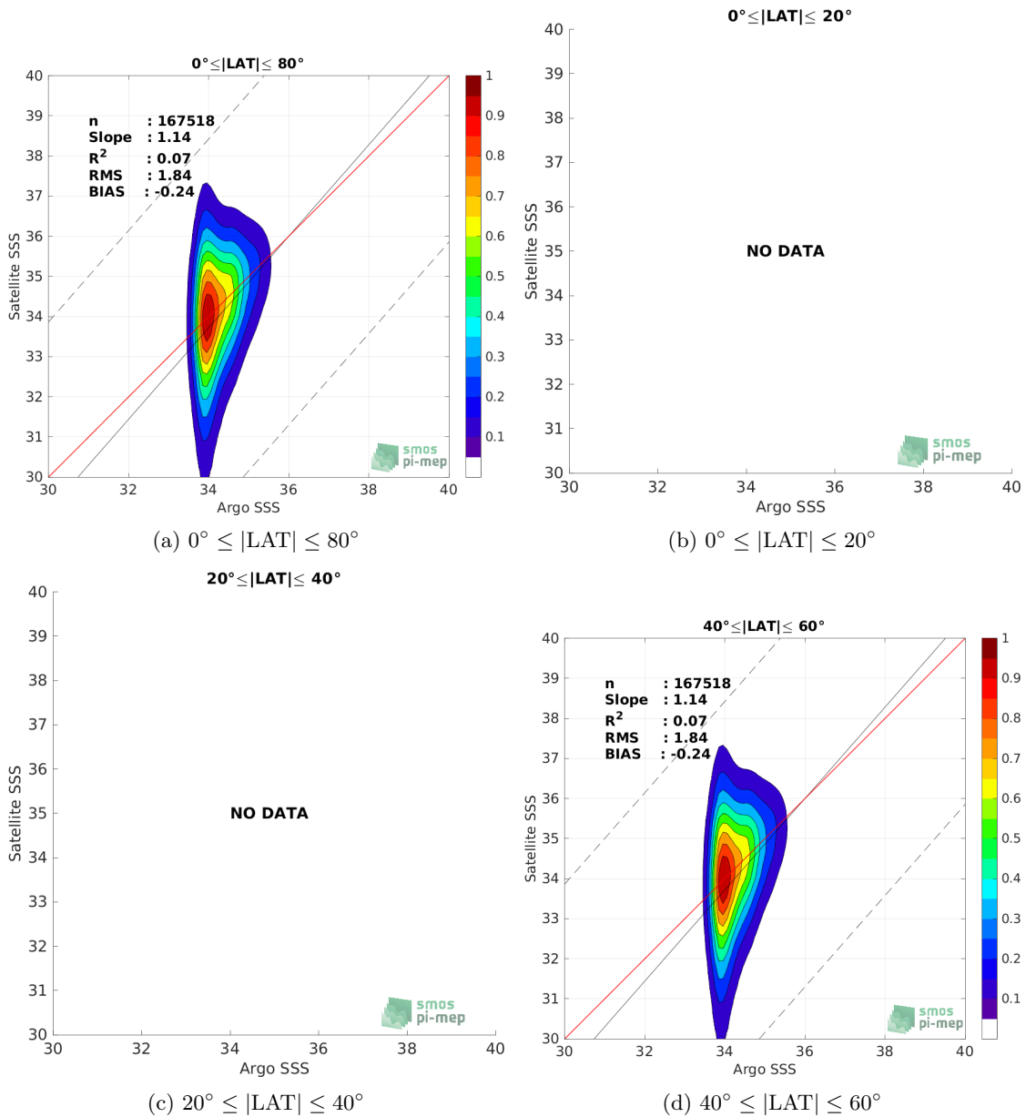
Figure 9: Contour maps of the concentration of SMOS SSS L2Q v331 - No FLAG (CMEMS-CATDS-CPDC) SSS (y-axis) versus Argo SSS (x-axis) at match-up pairs for different latitude bands. For each plot, the red line shows x=y . The black thin and dashed lines indicate a linear fit through the data cloud and the \pm 95\% confidence levels, respectively. The number match-up pairs n , the slope and R^2 coefficient of the linear fit, the root mean square (RMS) and the mean bias between satellite and in situ data are indicated for each latitude band in each plots.
