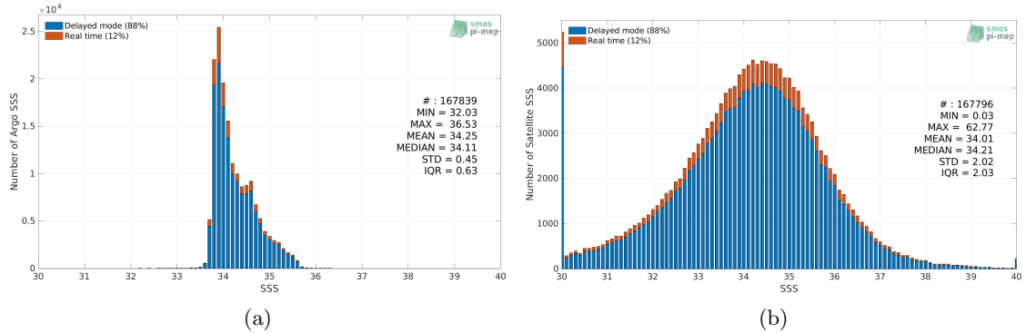
Figure 2: Histograms of SSS from Argo (a) and SMOS SSS L2Q v331 - No FLAG (CMEMS-CATDS-CPDC) (b) considering all match-up pairs per bins of 0.1 over the Roaring Forties and Furious Fifties Pi-MEP region and for the full satellite product period.
