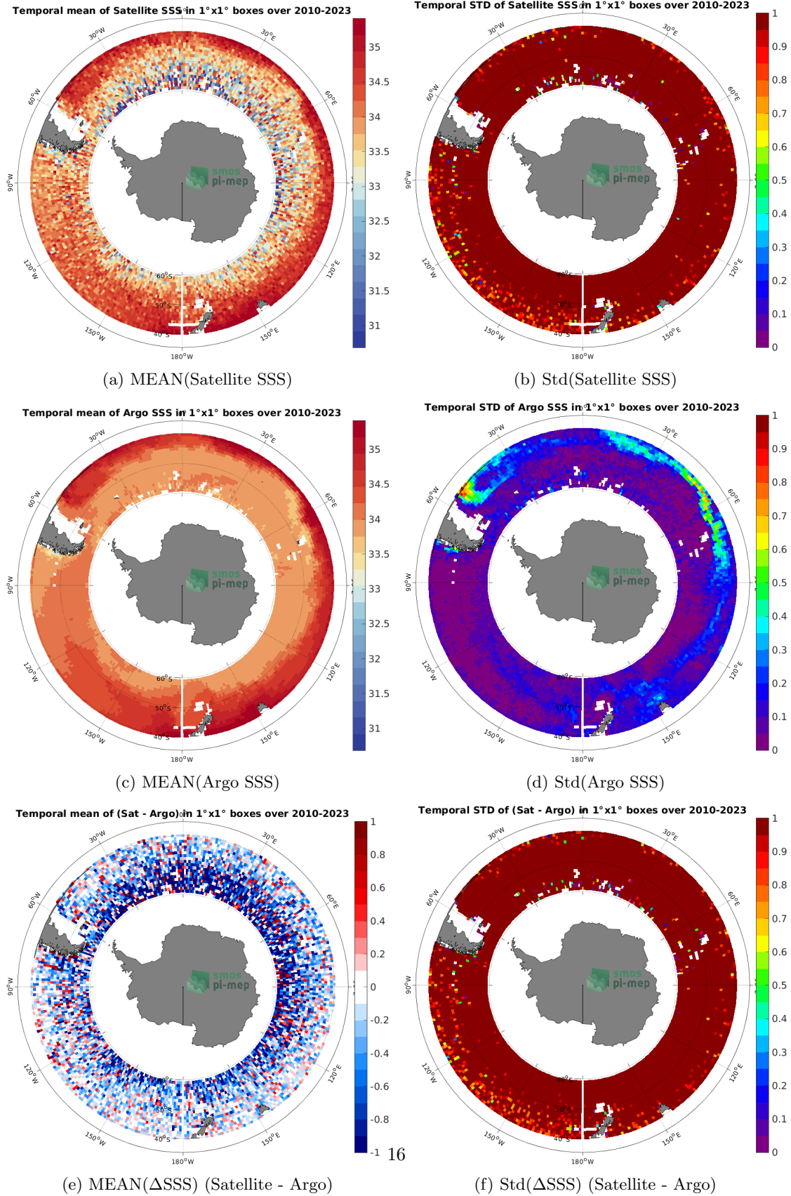
Figure 6: Temporal mean (left) and Std (right) of SSS from SMOS SSS L2Q v331 - No FLAG (CMEMS-CATDS-CPDC) (top), Argo (middle), and of \Delta SSS (Satellite - Argo). Only match-up pairs are used to generate these maps.
