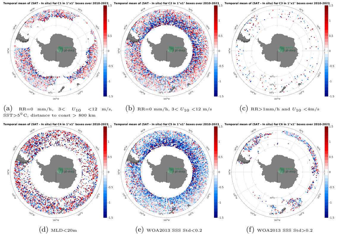
Figure 12: Temporal mean gridded over spatial boxes of size 1^{\circ}\times 1^{\circ} of \Delta\text{SSS} (SMOS SSS L2Q v331 - No FLAG (CMEMS-CATDS-CPDC) - Argo) for 6 different subdatasets corresponding to: RR=0 mm/h, 3 < U_{10} < 12 m/s, SST > 5^{\circ}\text{C} , distance to coast > 800 km (a), RR=0 mm/h, 3 < U_{10} < 12 m/s (b), RR > 1\text{mm/h} and U_{10} < 4\text{m/s} (c), MLD < 20\text{m} (d), WOA2013 SSS Std < 0.2 (e), WOA2013 SSS Std > 0.2 (f).
