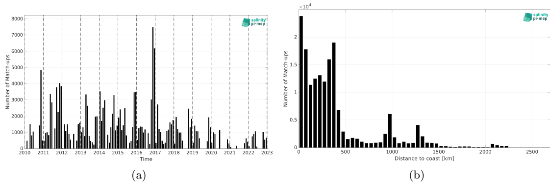
Figure 2: Number of match-ups between TSG (SAMOS) and SMOS SSS L3 v9 - 9 Days (CATDS-CEC-LOCEAN) SSS as a function of time (a) and as function of the distance to coast (b) over the Roaring Forties and Furious Fifties Pi-MEP region and for the full satellite product period.
