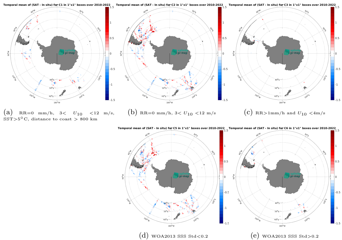
Figure 14: Temporal mean gridded over spatial boxes of size 1^\circ \times 1^\circ of \Delta\text{SSS} (SMOS SSS L3 v9 - 9 Days (CATDS-CEC-LOCEAN) - TSG (SAMOS)) for 5 different subdatasets corresponding to: RR=0 mm/h, 3 < U_{10} < 12 m/s, SST > 5°C, distance to coast > 800 km (a), RR=0 mm/h, 3 < U_{10} < 12 m/s (b), RR > 1mm/h and U_{10} < 4 m/s (c), WOA2013 SSS Std < 0.2 (d), WOA2013 SSS Std > 0.2 (e).
