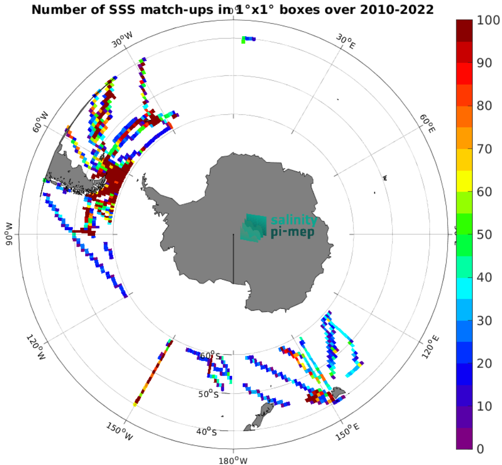
Figure 5: Number of SSS match-ups between TSG (SAMOS) SSS and the SMOS SSS L3 v9 - 9 Days (CATDS-CEC-LOCEAN) SSS product for the Roaring Forties and Furious Fifties Pi-MEP region over 1^\circ \times 1^\circ boxes and for the full satellite product period.
