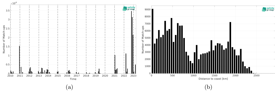
Figure 2: Number of match-ups between TSG (Polarstern) and SMOS SSS L3 v9 - 9 Days (CATDS-CEC-LOCEAN) SSS as a function of time (a) and as function of the distance to coast (b) over the Roaring Forties and Furious Fifties Pi-MEP region and for the full satellite product period.
