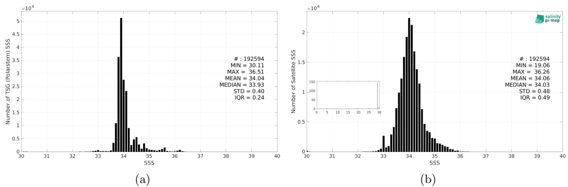
Figure 3: Histograms of SSS from TSG (Polarstern) (a) and SMOS SSS L3 v9 - 9 Days (CATDS-CEC-LOCEAN) (b) considering all match-up pairs per bins of 0.1 over the Roaring Forties and Furious Fifties Pi-MEP region and for the full satellite product period.
