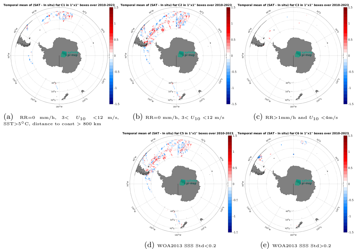
Figure 14: Temporal mean gridded over spatial boxes of size 1^\circ \times 1^\circ of \Delta SSS (SMOS SSS L3 v9 - 9 Days (CATDS-CEC-LOCEAN) - TSG (Polarstern)) for 5 different subdatasets corresponding to:RR=0 mm/h, 3 < U_{10} < 12 m/s, SST >5^\circ C, distance to coast > 800 km (a), RR=0 mm/h, 3 < U_{10} < 12 m/s (b), RR >1 mm/h and U_{10} < 4 m/s (c), WOA2013 SSS Std <0.2 (d), WOA2013 SSS Std >0.2 (e).
