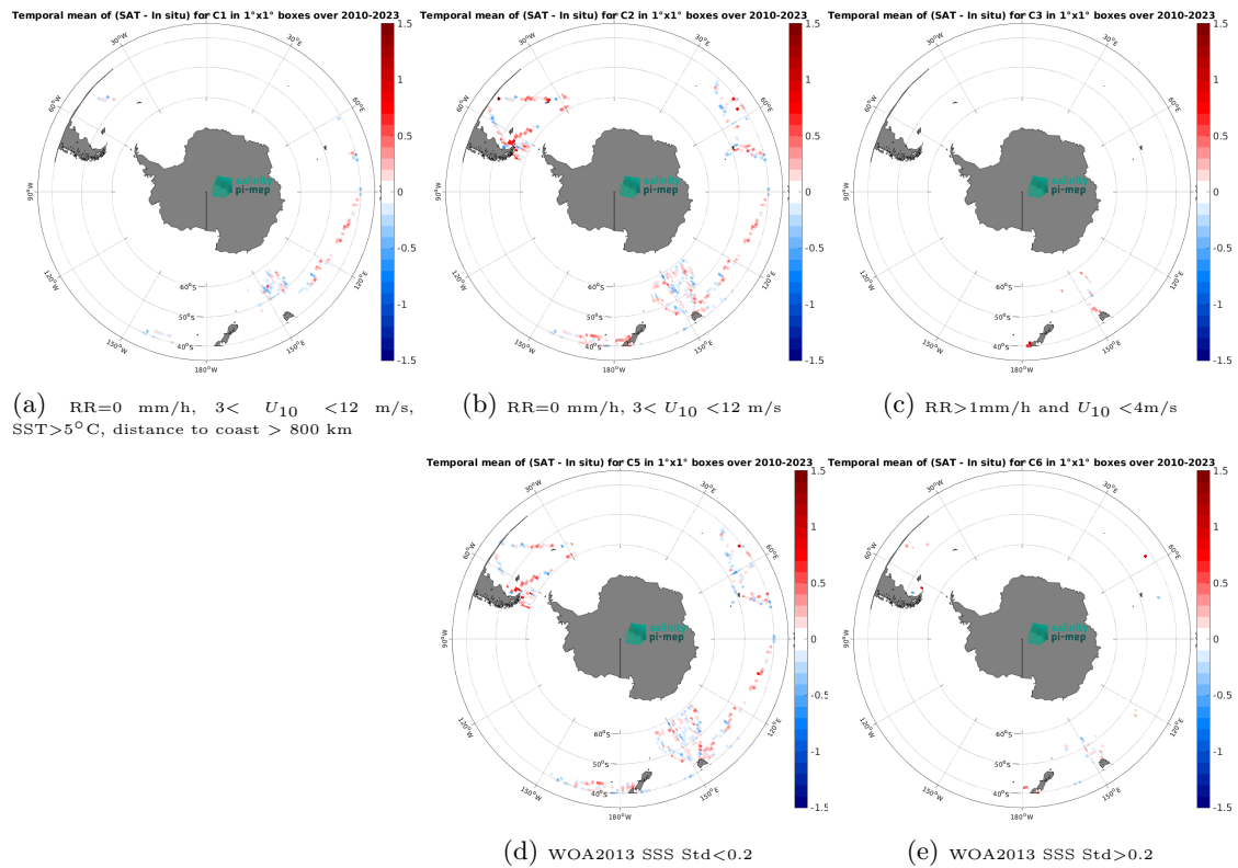
Figure 14: Temporal mean gridded over spatial boxes of size 1^\circ \times 1^\circ of \Delta\text{SSS} (SMOS SSS L3 v9 - 9 Days (CATDS-CEC-LOCEAN) - TSG (LEGOS-DM)) for 5 different subdatasets corresponding to: RR=0 mm/h, 3 < U_{10} < 12 m/s, SST > 5^\circ\text{C} , distance to coast > 800 km (a), RR=0 mm/h, 3 < U_{10} < 12 m/s (b), RR > 1 mm/h and U_{10} < 4 m/s (c), WOA2013 SSS Std < 0.2 (d), WOA2013 SSS Std > 0.2 (e).
