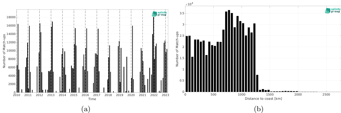
Figure 2: Number of match-ups between TSG (LEGOS-DM) and SMOS SSS L3 v9 - 9 Days (CATDS-CEC-LOCEAN) SSS as a function of time (a) and as function of the distance to coast (b) over the Roaring Forties and Furious Fifties Pi-MEP region and for the full satellite product period.
