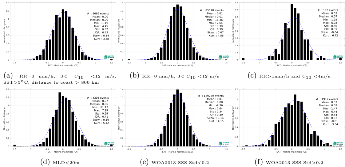
Figure 15: Normalized histogram of \Delta SSS (SMOS SSS L3 v9 - 9 Days (CATDS-CEC-LOCEAN) - Marine mammals) for 6 different subdatasets corresponding to: RR=0 mm/h, 3 < U_{10} < 12 m/s, SST > 5°C, distance to coast > 800 km (a), RR=0 mm/h, 3 < U_{10} < 12 m/s (b), RR > 1mm/h and U_{10} < 4 m/s (c), MLD < 20m (d), WOA2013 SSS Std < 0.2 (e), WOA2013 SSS Std > 0.2 (f).
