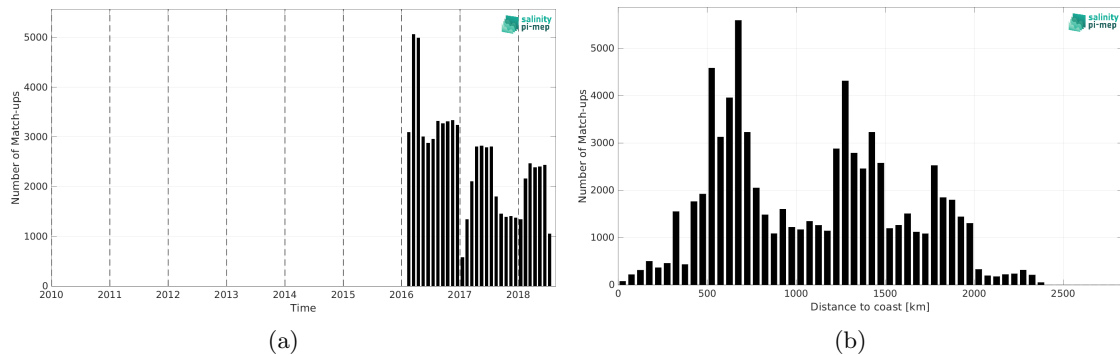
Figure 2: Number of match-ups between Surface drifters and SMOS SSS L3 v9 - 9 Days (CATDS-CEC-LOCEAN) SSS as a function of time (a) and as function of the distance to coast (b) over the Roaring Forties and Furious Fifties Pi-MEP region and for the full satellite product period.
