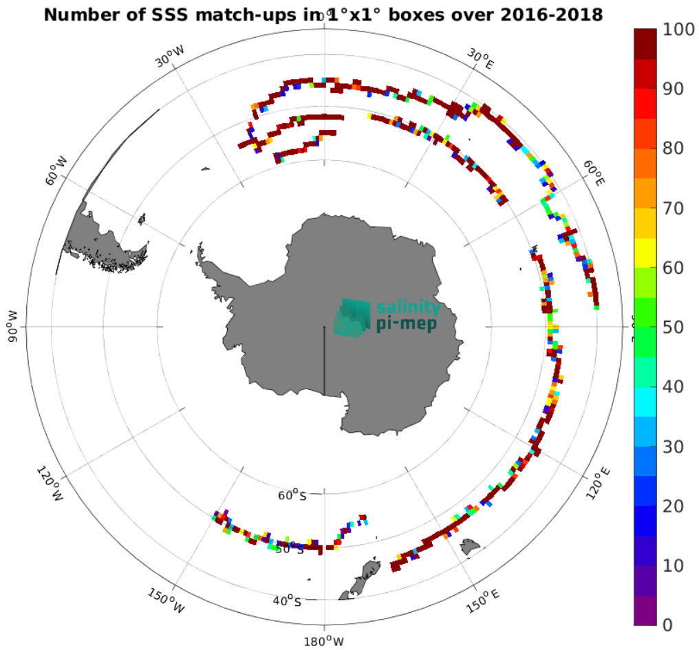
Figure 4: Number of SSS match-ups between Surface drifters SSS and the SMOS SSS L3 v9 - 9 Days (CATDS-CEC-LOCEAN) SSS product for the Roaring Forties and Furious Fifties Pi-MEP region over 1^\circ \times 1^\circ boxes and for the full satellite product period.
