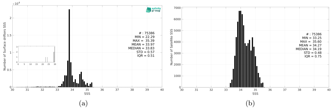
Figure 3: Histograms of SSS from Surface drifters (a) and SMOS SSS L3 v9 - 9 Days (CATDS-CEC-LOCEAN) (b) considering all match-up pairs per bins of 0.1 over the Roaring Forties and Furious Fifties Pi-MEP region and for the full satellite product period.
