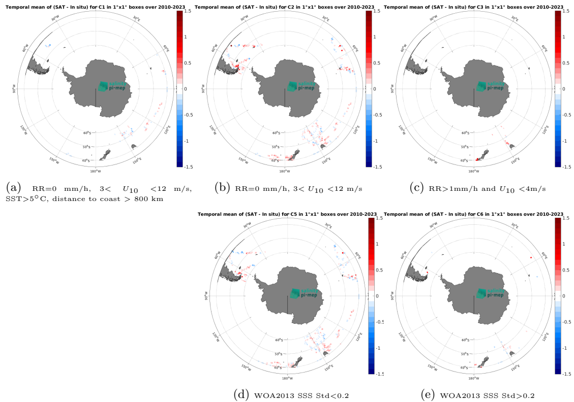
Figure 14: Temporal mean gridded over spatial boxes of size 1^\circ \times 1^\circ of \Delta\text{SSS} (SMOS SSS L3 v9 - 18 Days (CATDS-CEC-LOCEAN) - TSG (LEGOS-DM)) for 5 different subdatasets corresponding to: RR=0 mm/h, 3 < U_{10} < 12 m/s, SST > 5^\circ\text{C} , distance to coast > 800 km (a), RR=0 mm/h, 3 < U_{10} < 12 m/s (b), RR > 1 mm/h and U_{10} < 4 m/s (c), WOA2013 SSS Std < 0.2 (d), WOA2013 SSS Std > 0.2 (e).
