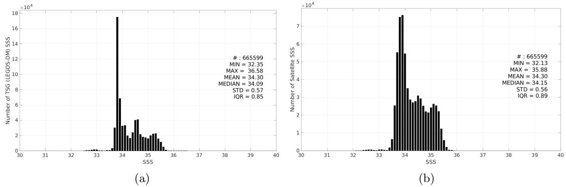
Figure 3: Histograms of SSS from TSG (LEGOS-DM) (a) and SMOS SSS L3 v9 - 18 Days (CATDS-CEC-LOCEAN) (b) considering all match-up pairs per bins of 0.1 over the Roaring Forties and Furious Fifties Pi-MEP region and for the full satellite product period.
