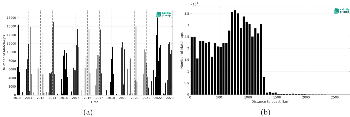
Figure 2: Number of match-ups between TSG (LEGOS-DM) and SMOS SSS L3 v9 - 18 Days (CATDS-CEC-LOCEAN) SSS as a function of time (a) and as function of the distance to coast (b) over the Roaring Forties and Furious Fifties Pi-MEP region and for the full satellite product period.
