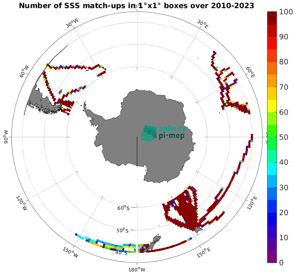
Figure 5: Number of SSS match-ups between TSG (LEGOS-DM) SSS and the SMOS SSS L3 v9 - 18 Days (CATDS-CEC-LOCEAN) SSS product for the Roaring Forties and Furious Fifties Pi-MEP region over 1^\circ \times 1^\circ boxes and for the full satellite product period.
