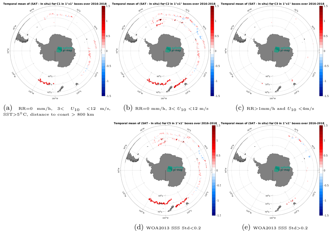
Figure 13: Temporal mean gridded over spatial boxes of size 1^\circ \times 1^\circ of \Delta SSS (SMOS SSS L3 v9 - 18 Days (CATDS-CEC-LOCEAN) - Surface drifters) for 5 different subdatasets corresponding to:RR=0 mm/h, 3 < U_{10} < 12 m/s, SST >5^\circ C, distance to coast > 800 km (a), RR=0 mm/h, 3 < U_{10} < 12 m/s (b), RR >1 mm/h and U_{10} < 4 m/s (c), WOA2013 SSS Std <0.2 (d), WOA2013 SSS Std >0.2 (e).
