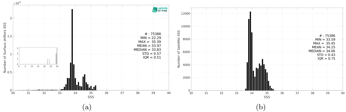
Figure 3: Histograms of SSS from Surface drifters (a) and SMOS SSS L3 v9 - 18 Days (CATDS-CEC-LOCEAN) (b) considering all match-up pairs per bins of 0.1 over the Roaring Forties and Furious Fifties Pi-MEP region and for the full satellite product period.
