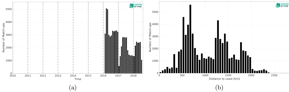
Figure 2: Number of match-ups between Surface drifters and SMOS SSS L3 v9 - 18 Days (CATDS-CEC-LOCEAN) SSS as a function of time (a) and as function of the distance to coast (b) over the Roaring Forties and Furious Fifties Pi-MEP region and for the full satellite product period.
