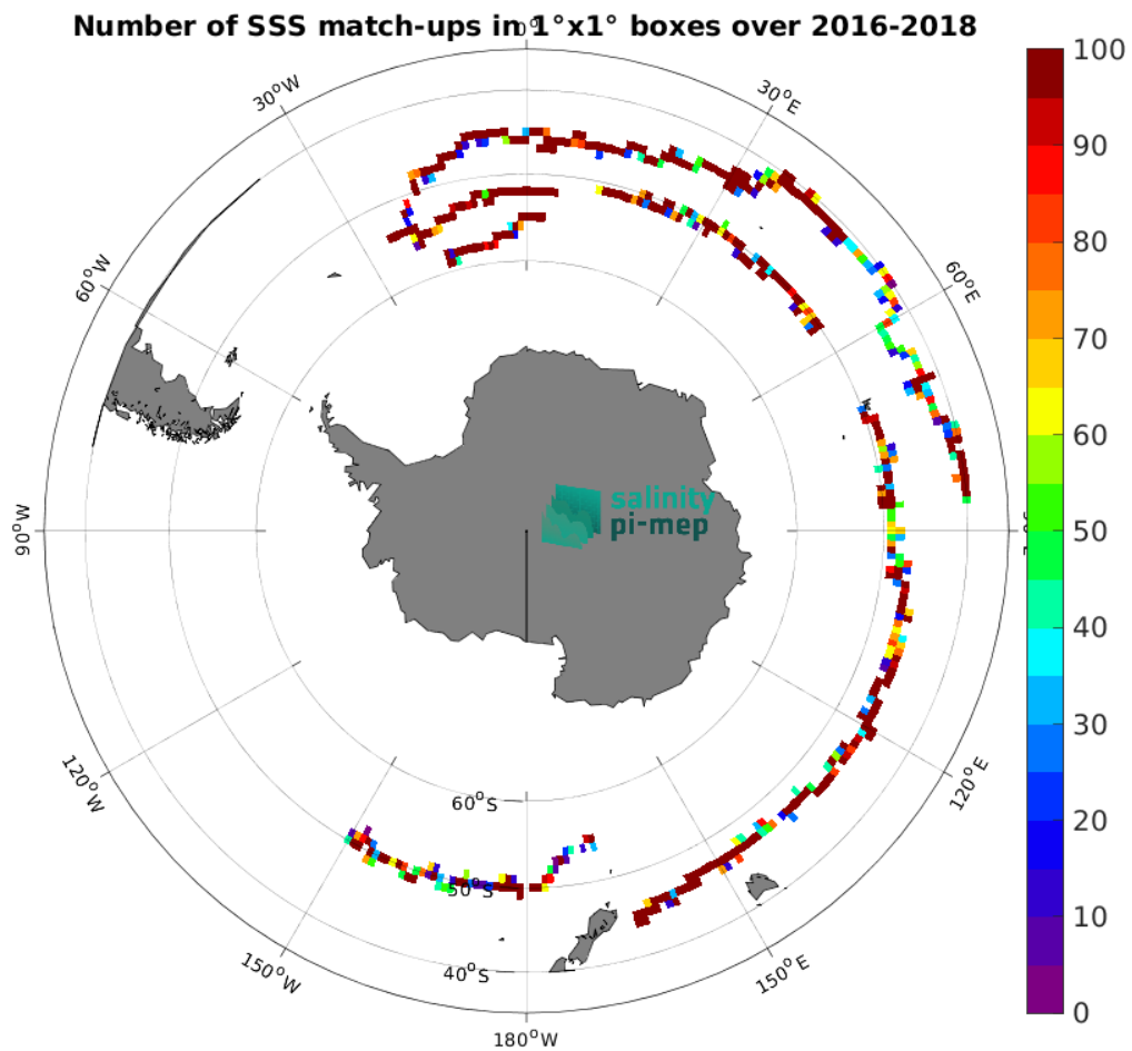
Figure 4: Number of SSS match-ups between Surface drifters SSS and the SMOS SSS L3 v9 - 18 Days (CATDS-CEC-LOCEAN) SSS product for the Roaring Forties and Furious Fifties Pi-MEP region over 1^\circ \times 1^\circ boxes and for the full satellite product period.
