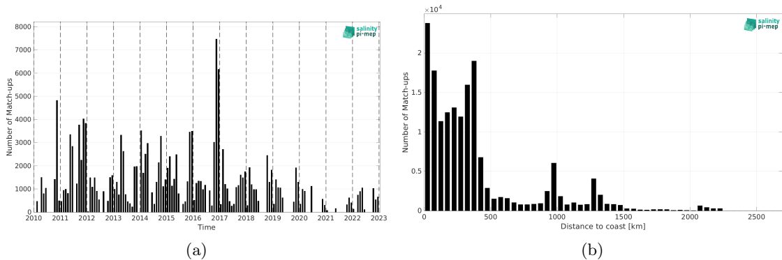
Figure 1: Number of match-ups between TSG (SAMOS) and SMOS SSS L3 v8 - 9 Days (CATDS-CEC-LOCEAN) SSS as a function of time (a) and as function of the distance to coast (b) over the Roaring Forties and Furious Fifties Pi-MEP region and for the full satellite product period.
