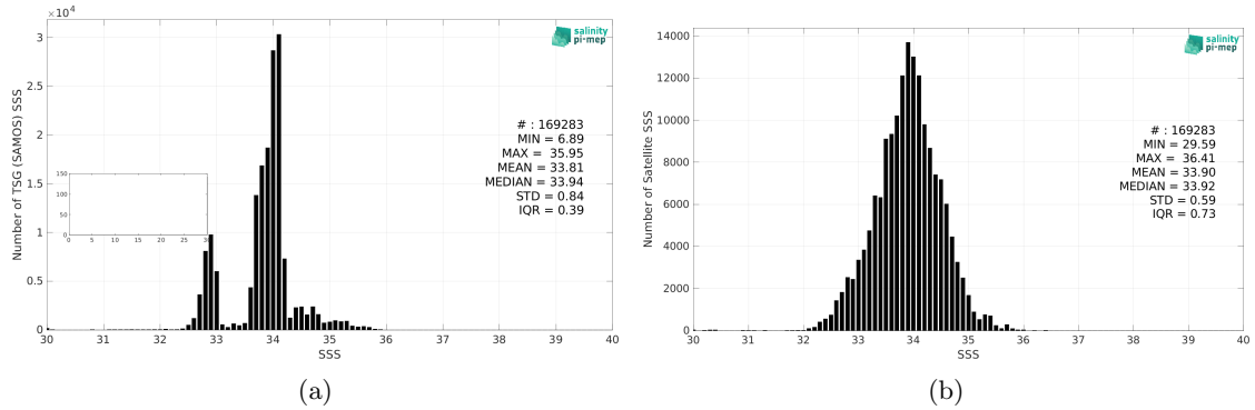
Figure 2: Histograms of SSS from TSG (SAMOS) (a) and SMOS SSS L3 v8 - 9 Days (CATDS-CEC-LOCEAN) (b) considering all match-up pairs per bins of 0.1 over the Roaring Forties and Furious Fifties Pi-MEP region and for the full satellite product period.
