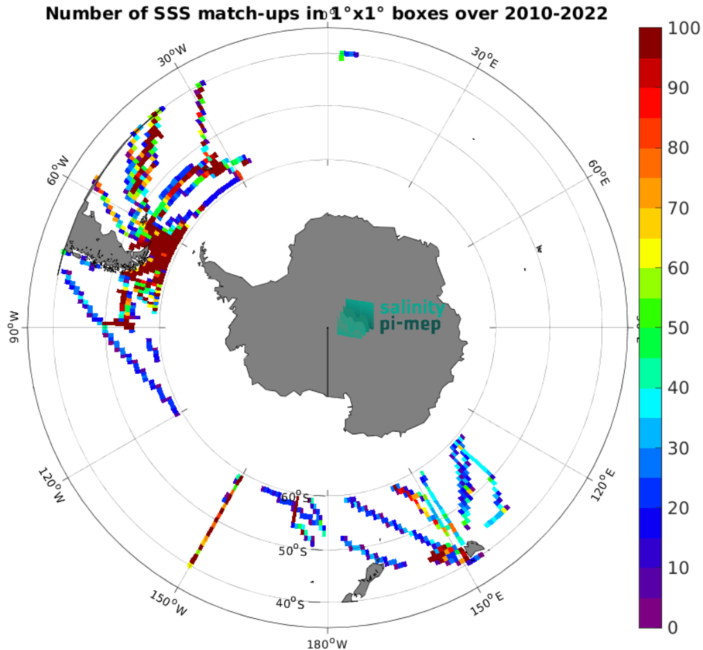
Figure 4: Number of SSS match-ups between TSG (SAMOS) SSS and the SMOS SSS L3 v8 - 9 Days (CATDS-CEC-LOCEAN) SSS product for the Roaring Forties and Furious Fifties Pi-MEP region over 1^\circ \times 1^\circ boxes and for the full satellite product period.
