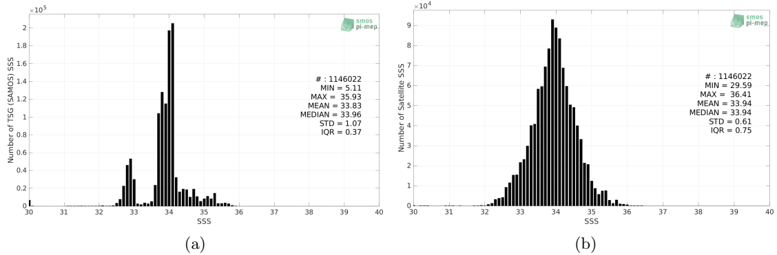
Figure 2: Histograms of SSS from TSG (SAMOS) (a) and SMOS SSS L3 v8 - 9 Days (CATDS-CECOS-LOCEAN) (b) considering all match-up pairs per bins of 0.1 over the Roaring Forties and Furious Fifties Pi-MEP region and for the full satellite product period.
