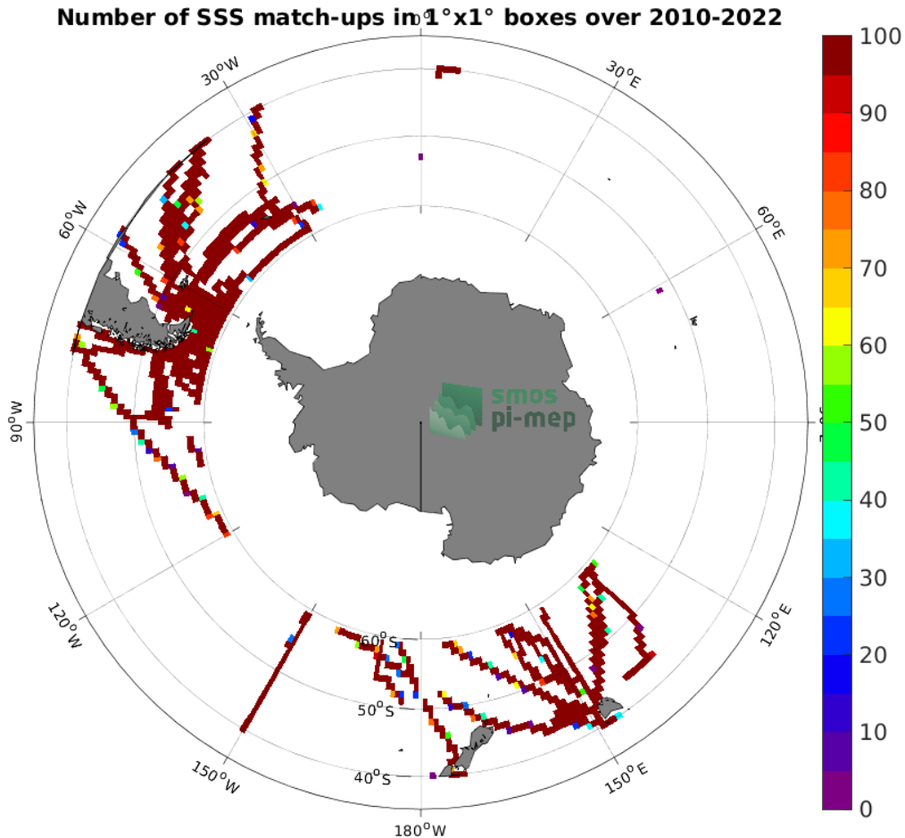
Figure 4: Number of SSS match-ups between TSG (SAMOS) SSS and the SMOS SSS L3 v8 - 9 Days (CATDS-CECOS-LOCEAN) SSS product for the Roaring Forties and Furious Fifties Pi-MEP region over 1^\circ \times 1^\circ boxes and for the full satellite product period.
