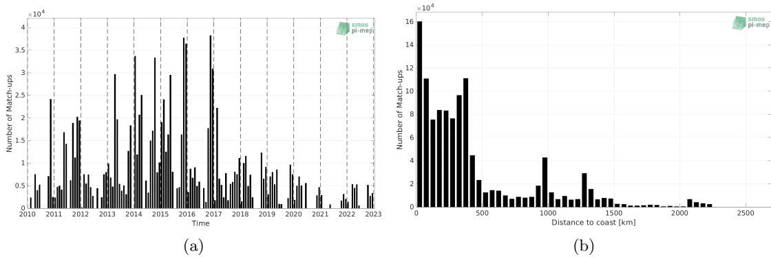
Figure 1: Number of match-ups between TSG (SAMOS) and SMOS SSS L3 v8 - 9 Days (CATDS-CECOS-LOCEAN) SSS as a function of time (a) and as function of the distance to coast (b) over the Roaring Forties and Furious Fifties Pi-MEP region and for the full satellite product period.
