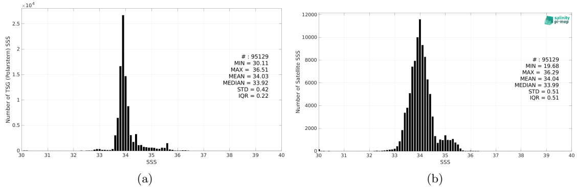
Figure 2: Histograms of SSS from TSG (Polarstern) (a) and SMOS SSS L3 v8 - 9 Days (CATDS-CEC-LOCEAN) (b) considering all match-up pairs per bins of 0.1 over the Roaring Forties and Furious Fifties Pi-MEP region and for the full satellite product period.
