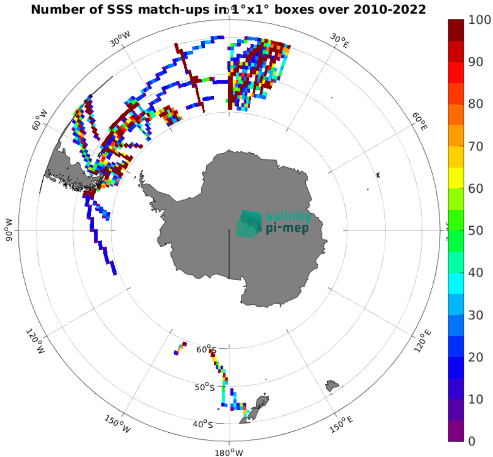
Figure 4: Number of SSS match-ups between TSG (Polarstern) SSS and the SMOS SSS L3 v8 - 9 Days (CATDS-CEC-LOCEAN) SSS product for the Roaring Forties and Furious Fifties Pi-MEP region over 1^\circ \times 1^\circ boxes and for the full satellite product period.
