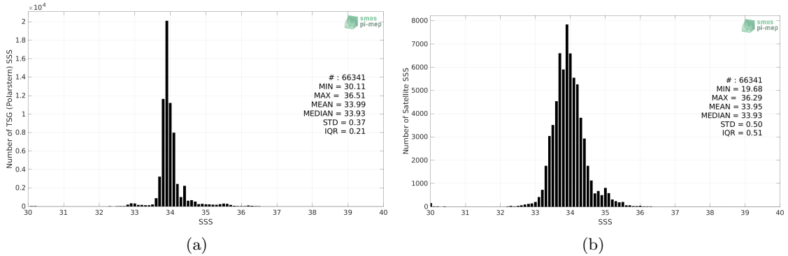
Figure 2: Histograms of SSS from TSG (Polarstern) (a) and SMOS SSS L3 v8 - 9 Days (CATDS-CECOS-LOCEAN) (b) considering all match-up pairs per bins of 0.1 over the Roaring Forties and Furious Fifties Pi-MEP region and for the full satellite product period.
