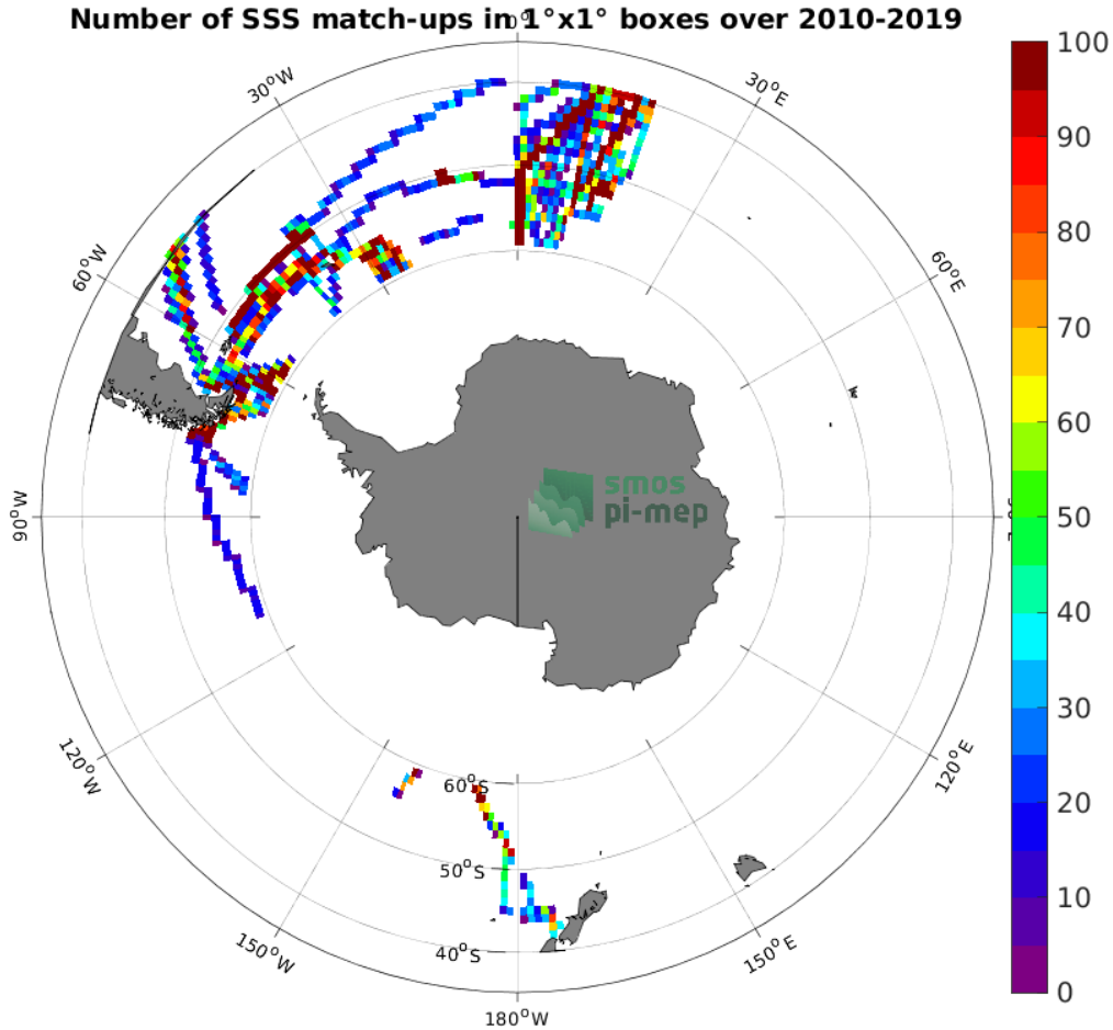
Figure 4: Number of SSS match-ups between TSG (Polarstern) SSS and the SMOS SSS L3 v8 - 9 Days (CATDS-CECOS-LOCEAN) SSS product for the Roaring Forties and Furious Fifties Pi-MEP region over 1^\circ \times 1^\circ boxes and for the full satellite product period.
