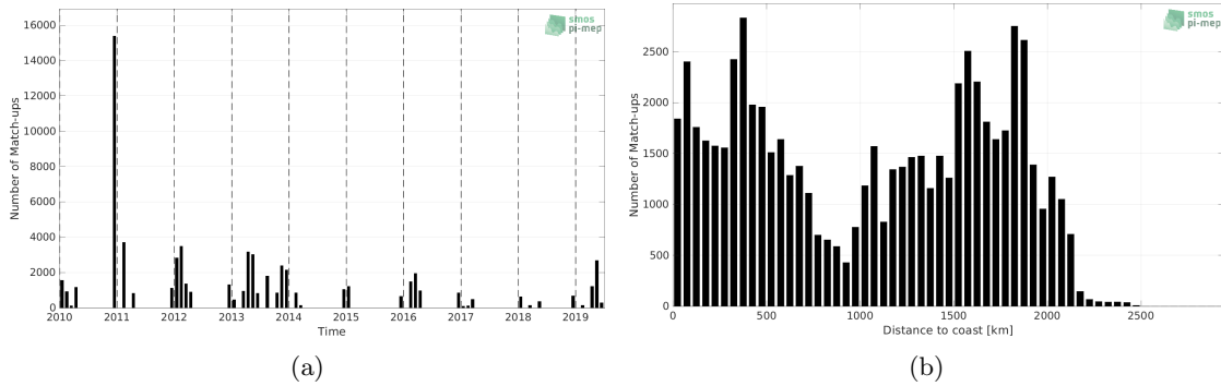
Figure 1: Number of match-ups between TSG (Polarstern) and SMOS SSS L3 v8 - 9 Days (CATDS-CECOS-LOCEAN) SSS as a function of time (a) and as function of the distance to coast (b) over the Roaring Forties and Furious Fifties Pi-MEP region and for the full satellite product period.
