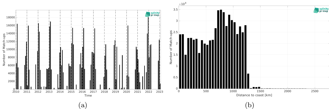
Figure 1: Number of match-ups between TSG (LEGOS-DM) and SMOS SSS L3 v8 - 9 Days (CATDS-CEC-LOCEAN) SSS as a function of time (a) and as function of the distance to coast (b) over the Roaring Forties and Furious Fifties Pi-MEP region and for the full satellite product period.
