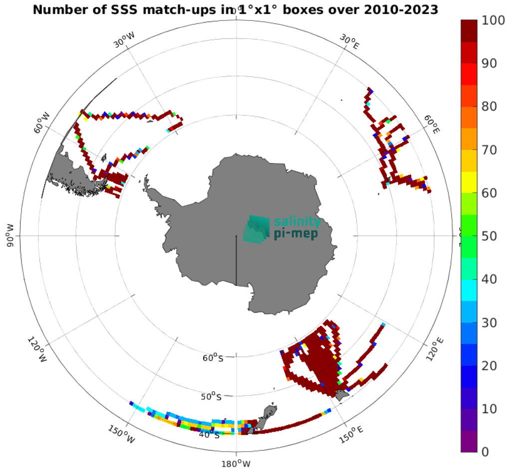
Figure 4: Number of SSS match-ups between TSG (LEGOS-DM) SSS and the SMOS SSS L3 v8 - 9 Days (CATDS-CEC-LOCEAN) SSS product for the Roaring Forties and Furious Fifties Pi-MEP region over 1^\circ \times 1^\circ boxes and for the full satellite product period.
