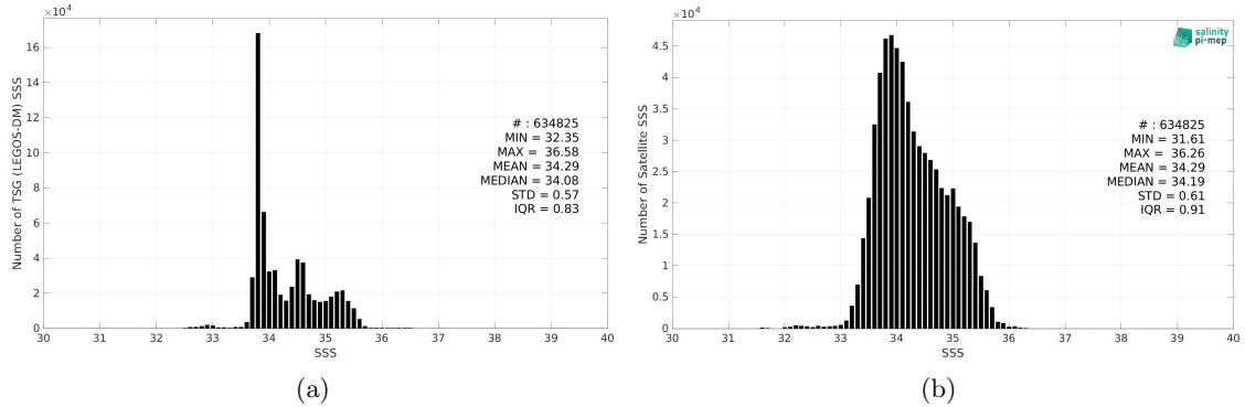
Figure 2: Histograms of SSS from TSG (LEGOS-DM) (a) and SMOS SSS L3 v8 - 9 Days (CATDS-CEC-LOCEAN) (b) considering all match-up pairs per bins of 0.1 over the Roaring Forties and Furious Fifties Pi-MEP region and for the full satellite product period.
