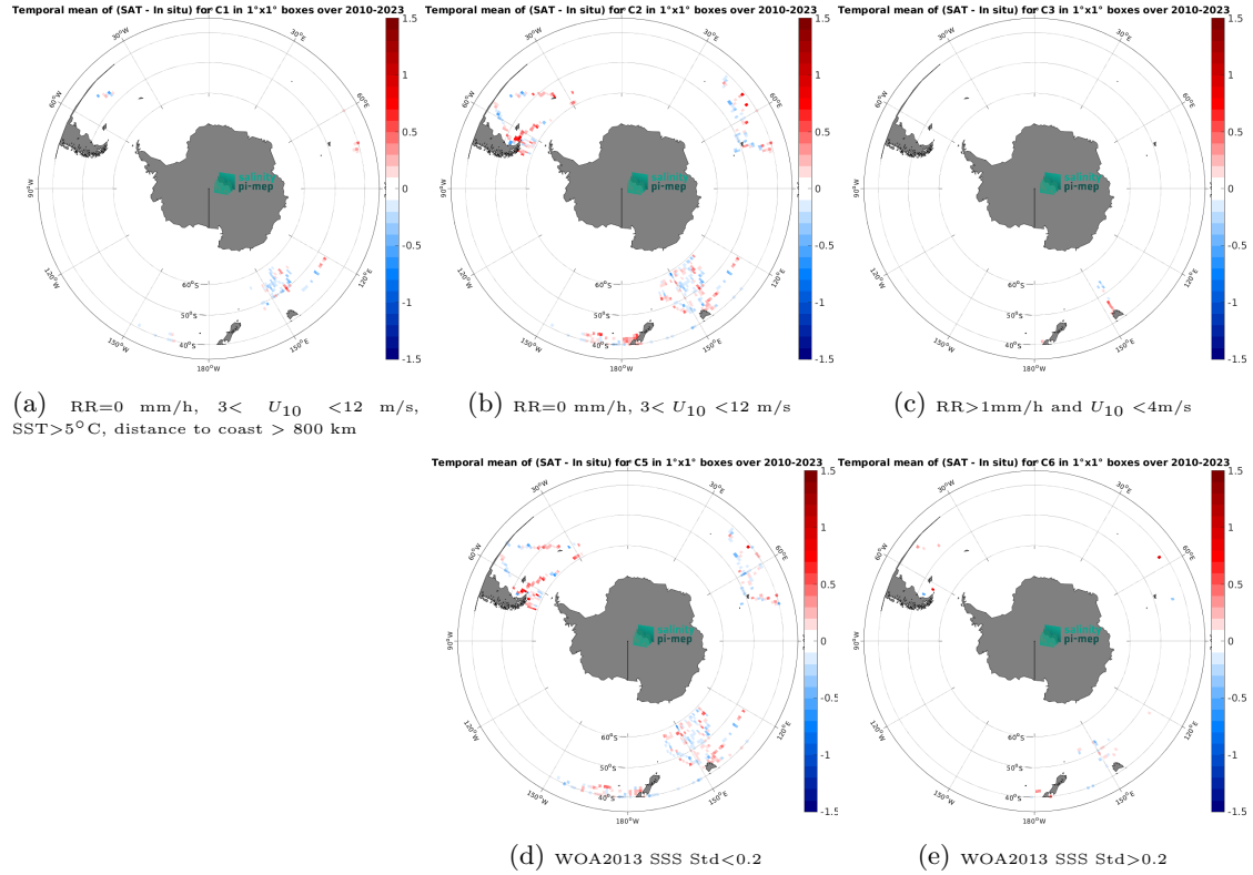
Figure 12: Temporal mean gridded over spatial boxes of size 1^{\circ}\times 1^{\circ} of \Delta\text{SSS} (SMOS SSS L3 v8 - 9 Days (CATDS-CEC-LOCEAN) - TSG (LEGOS-DM)) for 5 different subdatasets corresponding to: \text{RR}=0 mm/h, 3 < U_{10} < 12 m/s, \text{SST}>5^{\circ}\text{C} , distance to coast > 800 km (a), \text{RR}=0 mm/h, 3 < U_{10} < 12 m/s (b), \text{RR}>1 mm/h and U_{10} < 4 m/s (c), WOA2013 SSS Std <0.2 (d), WOA2013 SSS Std >0.2 (e).
