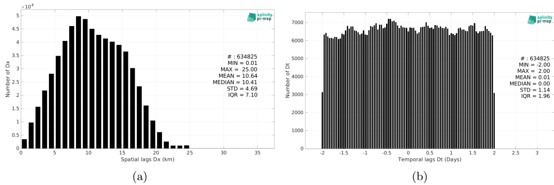
Figure 5: Histograms of the spatial (a) and temporal (b) lags between the location/time of the TSG (LEGOS-DM) measurement and the date of the corresponding SMOS SSS L3 v8 - 9 Days (CATDS-CEC-LOCEAN) SSS pixel.
