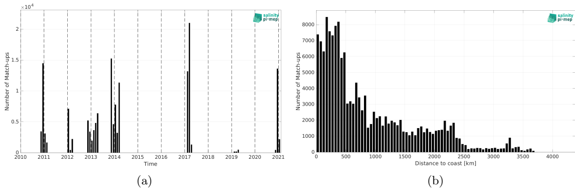
Figure 1: Number of match-ups between TSG (GOSUD-Sailing-ship) and SMOS SSS L3 v8 - 9 Days (CATDS-CEC-LOCEAN) SSS as a function of time (a) and as function of the distance to coast (b) over the Roaring Forties and Furious Fifties Pi-MEP region and for the full satellite product period.
