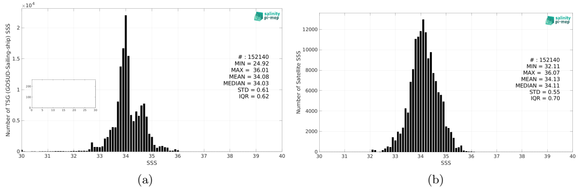
Figure 2: Histograms of SSS from TSG (GOSUD-Sailing-ship) (a) and SMOS SSS L3 v8 - 9 Days (CATDS-CEC-LOCEAN) (b) considering all match-up pairs per bins of 0.1 over the Roaring Forties and Furious Fifties Pi-MEP region and for the full satellite product period.
