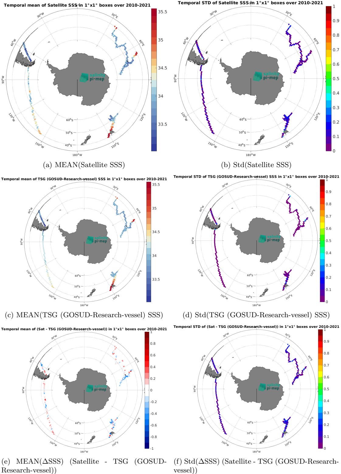
Figure 6: Temporal mean (left) and Std (right) of SSS from SMOS SSS L3 v8 - 9 Days (CATDS-CEC-LOCEAN) (top), TSG (GOSUD-Research-vessel) (middle), and of \Delta SSS (Satellite - TSG (GOSUD-Research-vessel)). Only match-up pairs are used to generate these maps.
