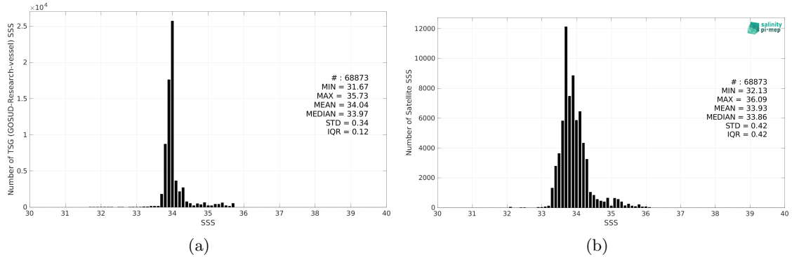
Figure 2: Histograms of SSS from TSG (GOSUD-Research-vessel) (a) and SMOS SSS L3 v8 - 9 Days (CATDS-CEC-LOCEAN) (b) considering all match-up pairs per bins of 0.1 over the Roaring Forties and Furious Fifties Pi-MEP region and for the full satellite product period.
