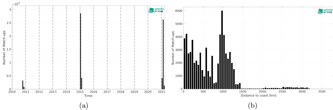
Figure 1: Number of match-ups between TSG (GOSUD-Research-vessel) and SMOS SSS L3 v8 - 9 Days (CATDS-CEC-LOCEAN) SSS as a function of time (a) and as function of the distance to coast (b) over the Roaring Forties and Furious Fifties Pi-MEP region and for the full satellite product period.
