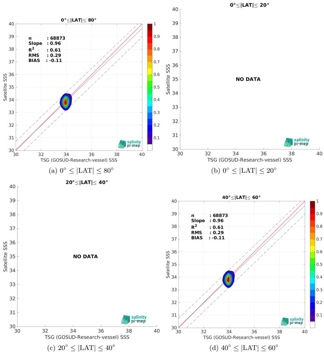
Figure 9: Contour maps of the concentration of SMOS SSS L3 v8 - 9 Days (CATDS-CEC-LOCEAN) SSS (y-axis) versus TSG (GOSUD-Research-vessel) SSS (x-axis) at match-up pairs for different latitude bands. For each plot, the red line shows x=y . The black thin and dashed lines indicate a linear fit through the data cloud and the \pm 95\% confidence levels, respectively. The number match-up pairs n , the slope and R^2 coefficient of the linear fit, the root mean square (RMS) and the mean bias between satellite and in situ data are indicated for each latitude band in each plots.
