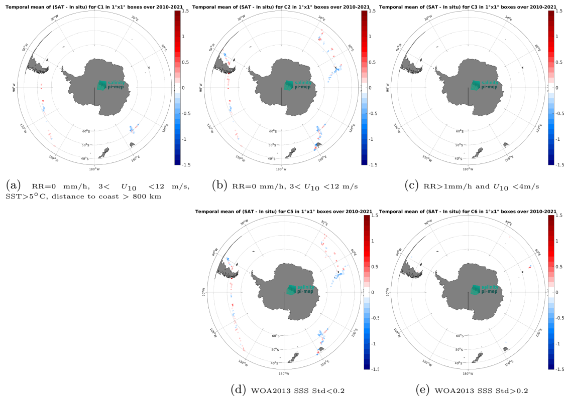
Figure 12: Temporal mean gridded over spatial boxes of size 1^\circ \times 1^\circ of \Delta SSS (SMOS SSS L3 v8 - 9 Days (CATDS-CEC-LOCEAN) - TSG (GOSUD-Research-vessel)) for 5 different subdatasets corresponding to:RR=0 mm/h, 3 < U_{10} < 12 m/s, SST>5°C, distance to coast > 800 km (a), RR=0 mm/h, 3 < U_{10} < 12 m/s (b), RR>1mm/h and U_{10} < 4 m/s (c), WOA2013 SSS Std<0.2 (d), WOA2013 SSS Std>0.2 (e).
