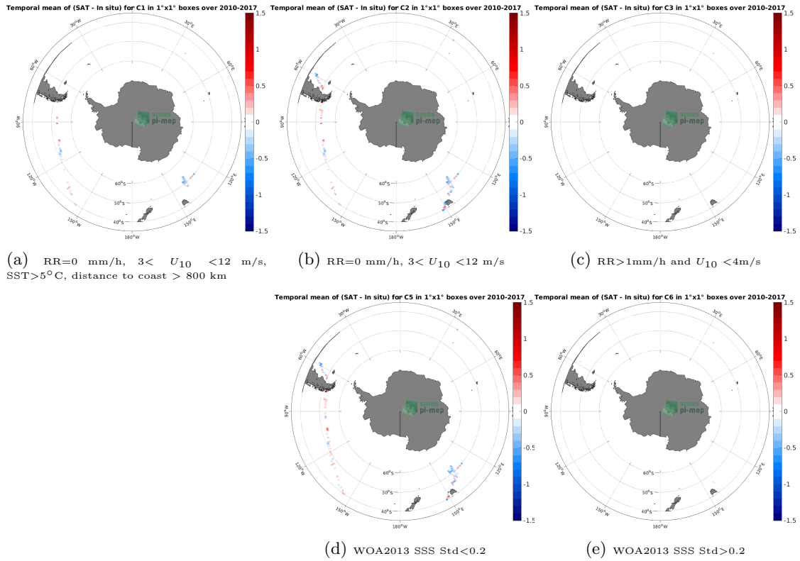
Figure 12: Temporal mean gridded over spatial boxes of size 1^\circ \times 1^\circ of \Delta SSS (SMOS SSS L3 v8 - 9 Days (CATDS-CECOS-LOCEAN) - TSG (GOSUD-Research-vessel)) for 5 different subdatasets corresponding to:RR=0 mm/h, 3 < U_{10} < 12 m/s, SST>5°C, distance to coast > 800 km (a), RR=0 mm/h, 3 < U_{10} < 12 m/s (b), RR>1mm/h and U_{10} < 4 m/s (c), WOA2013 SSS Std<0.2 (d), WOA2013 SSS Std>0.2 (e).
