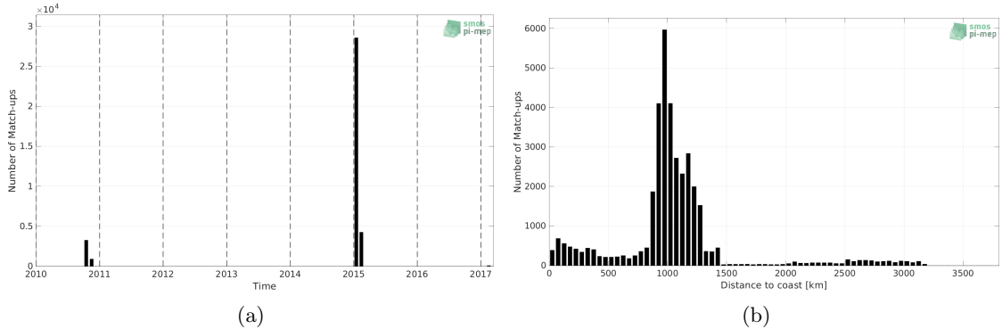
Figure 1: Number of match-ups between TSG (GOSUD-Research-vessel) and SMOS SSS L3 v8 - 9 Days (CATDS-CECOS-LOCEAN) SSS as a function of time (a) and as function of the distance to coast (b) over the Roaring Forties and Furious Fifties Pi-MEP region and for the full satellite product period.
