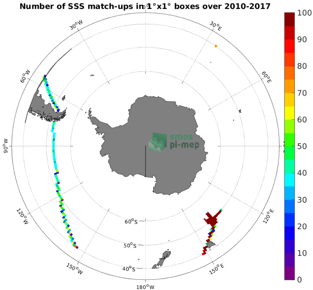
Figure 4: Number of SSS match-ups between TSG (GOSUD-Research-vessel) SSS and the SMOS SSS L3 v8 - 9 Days (CATDS-CECOS-LOCEAN) SSS product for the Roaring Forties and Furious Fifties Pi-MEP region over 1^\circ \times 1^\circ boxes and for the full satellite product period.
