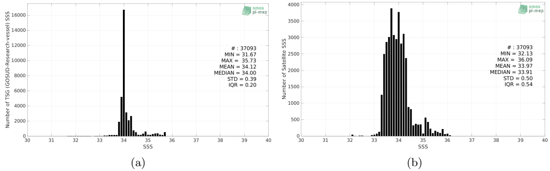
Figure 2: Histograms of SSS from TSG (GOSUD-Research-vessel) (a) and SMOS SSS L3 v8 - 9 Days (CATDS-CECOS-LOCEAN) (b) considering all match-up pairs per bins of 0.1 over the Roaring Forties and Furious Fifties Pi-MEP region and for the full satellite product period.
