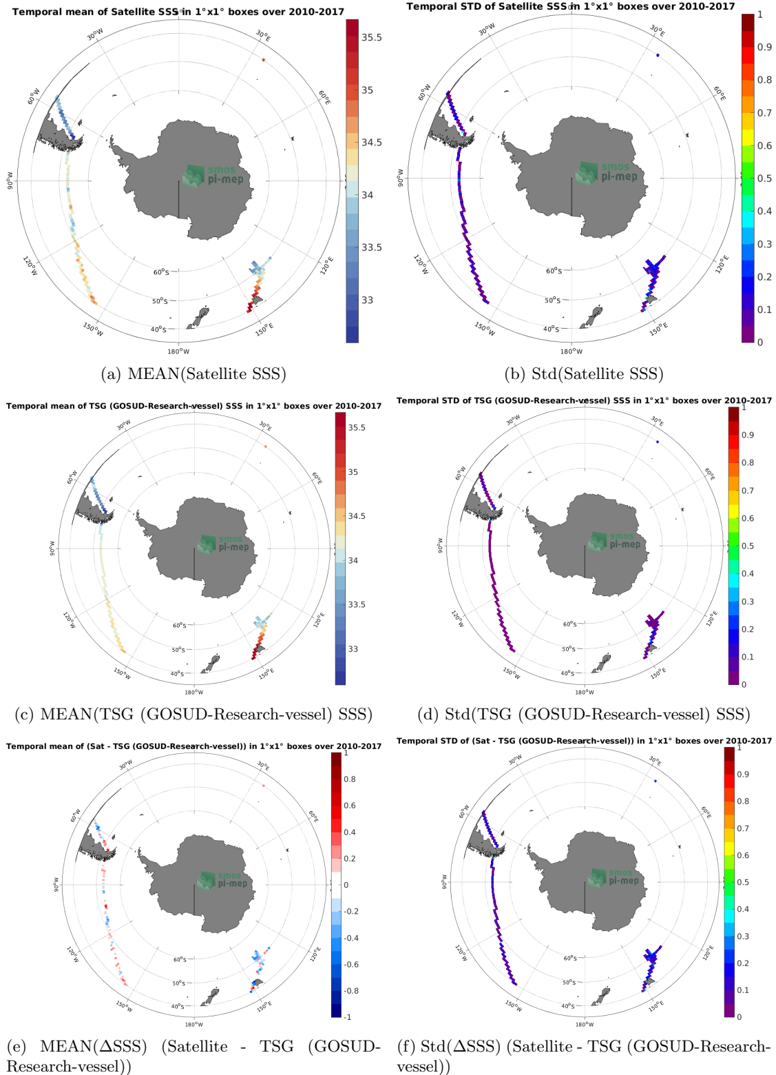
Figure 6: Temporal mean (left) and Std (right) of SSS from SMOS SSS L3 v8 - 9 Days (CATDS-CECOS-LOCEAN) (top), TSG (GOSUD-Research-vessel) (middle), and of \Delta SSS (Satellite - TSG (GOSUD-Research-vessel)). Only match-16 pairs are used to generate these maps.
