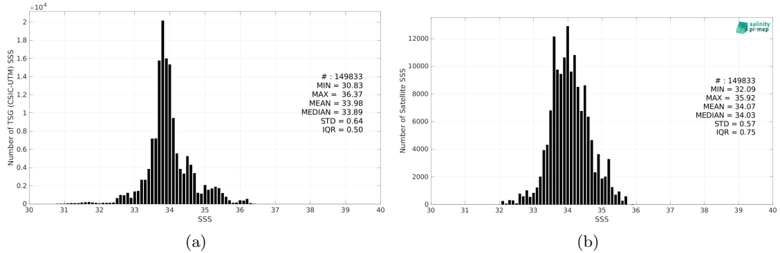
Figure 2: Histograms of SSS from TSG (CSIC-UTM) (a) and SMOS SSS L3 v8 - 9 Days (CATDS-CEC-LOCEAN) (b) considering all match-up pairs per bins of 0.1 over the Roaring Forties and Furious Fifties Pi-MEP region and for the full satellite product period.
