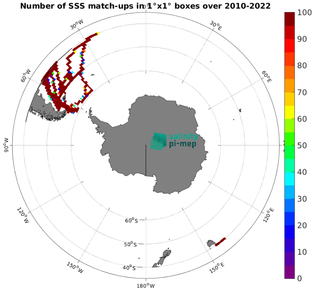
Figure 4: Number of SSS match-ups between TSG (CSIC-UTM) SSS and the SMOS SSS L3 v8 - 9 Days (CATDS-CEC-LOCEAN) SSS product for the Roaring Forties and Furious Fifties Pi-MEP region over 1^\circ \times 1^\circ boxes and for the full satellite product period.
