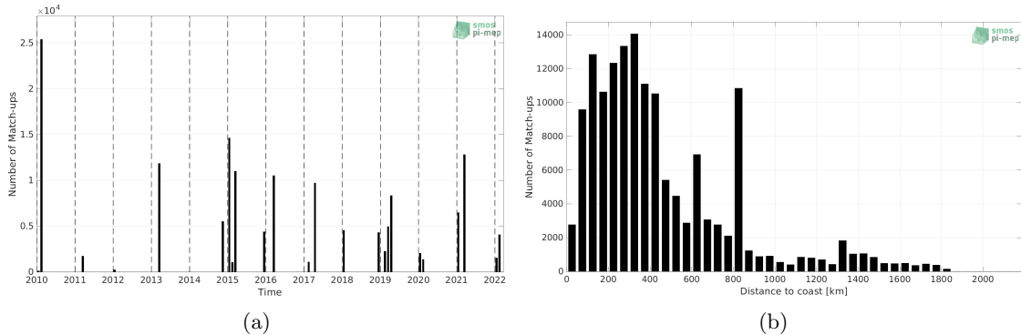
Figure 1: Number of match-ups between TSG (CSIC-UTM) and SMOS SSS L3 v8 - 9 Days (CATDS-CECOS-LOCEAN) SSS as a function of time (a) and as function of the distance to coast (b) over the Roaring Forties and Furious Fifties Pi-MEP region and for the full satellite product period.
