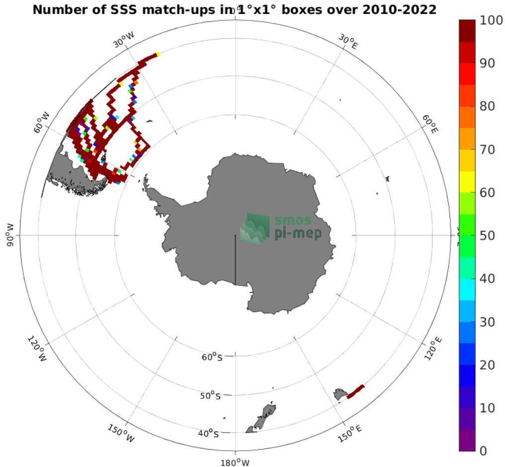
Figure 4: Number of SSS match-ups between TSG (CSIC-UTM) SSS and the SMOS SSS L3 v8 - 9 Days (CATDS-CECOS-LOCEAN) SSS product for the Roaring Forties and Furious Fifties Pi-MEP region over 1^\circ \times 1^\circ boxes and for the full satellite product period.
