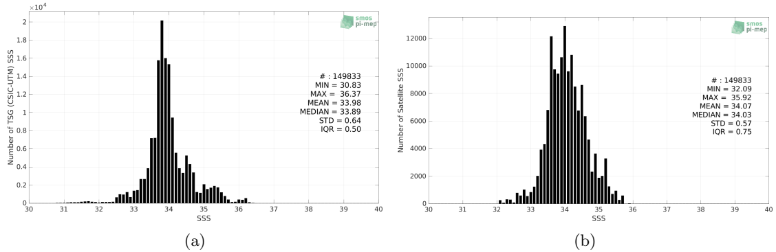
Figure 2: Histograms of SSS from TSG (CSIC-UTM) (a) and SMOS SSS L3 v8 - 9 Days (CATDS-CECOS-LOCEAN) (b) considering all match-up pairs per bins of 0.1 over the Roaring Forties and Furious Fifties Pi-MEP region and for the full satellite product period.
