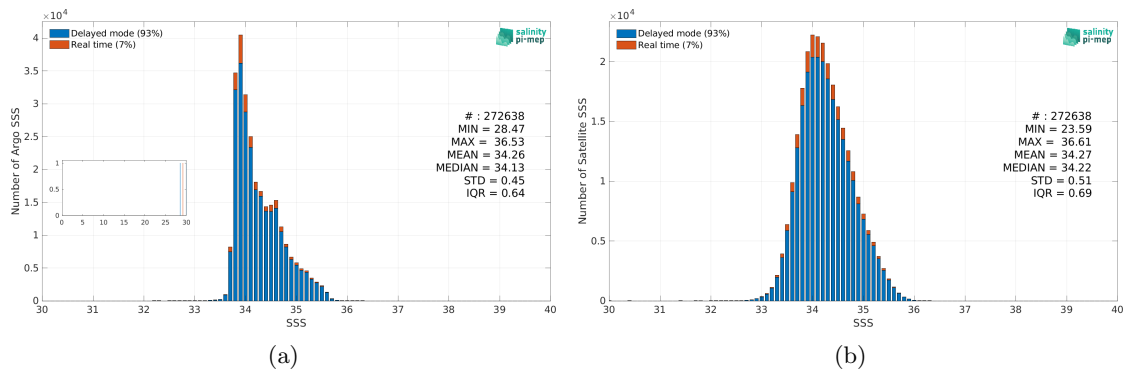
Figure 2: Histograms of SSS from Argo (a) and SMOS SSS L3 v8 - 9 Days (CATDS-CEC-LOCEAN) (b) considering all match-up pairs per bins of 0.1 over the Roaring Forties and Furious Fifties Pi-MEP region and for the full satellite product period.
