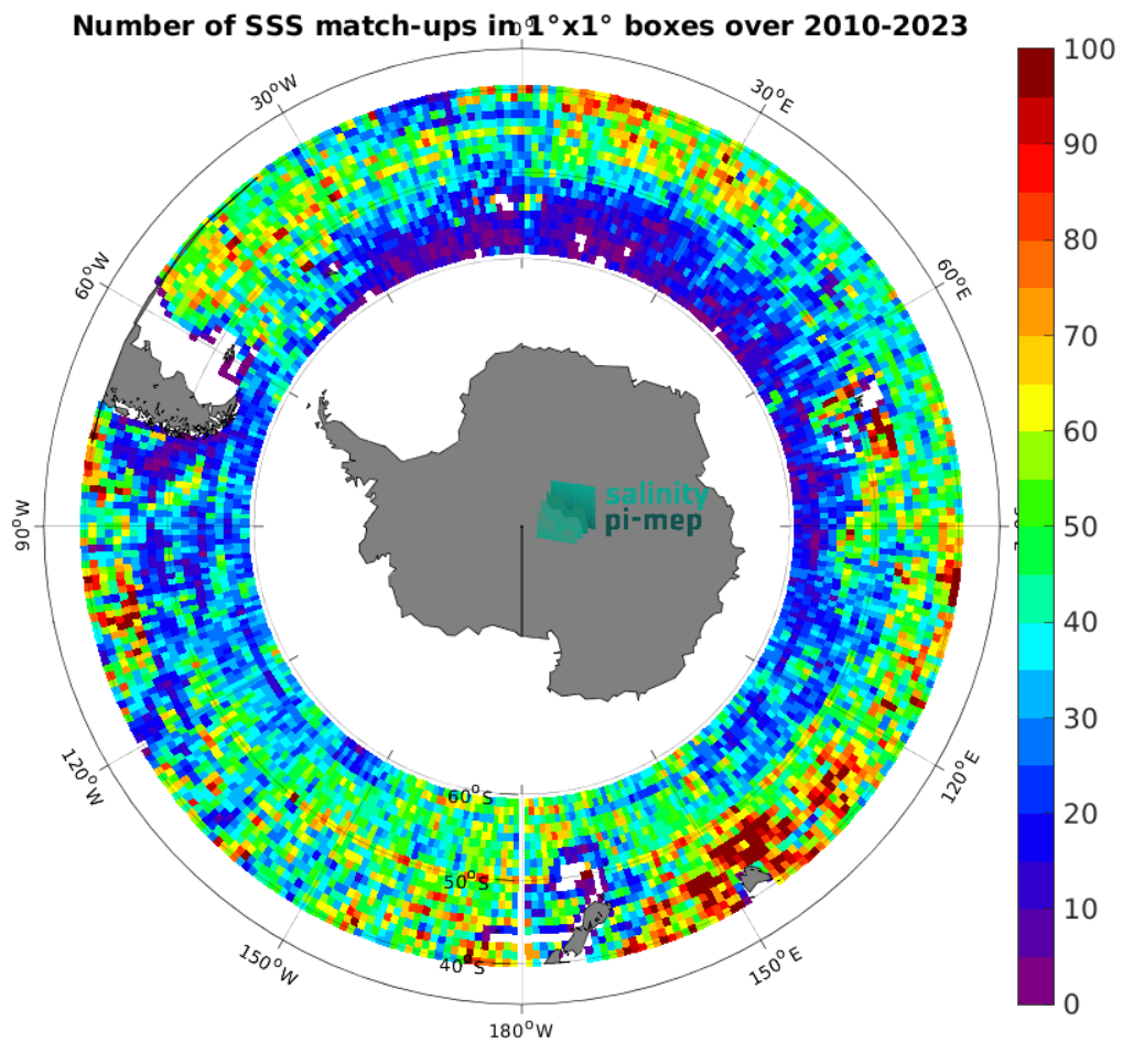
Figure 4: Number of SSS match-ups between Argo SSS and the SMOS SSS L3 v8 - 9 Days (CATDS-CEC-LOCEAN) SSS product for the Roaring Forties and Furious Fifties Pi-MEP region over 1^\circ \times 1^\circ boxes and for the full satellite product period.
