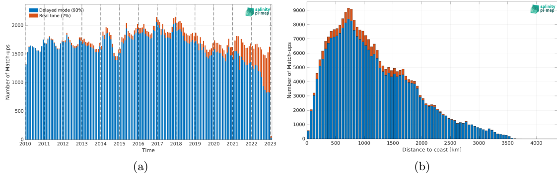
Figure 1: Number of match-ups between Argo and SMOS SSS L3 v8 - 9 Days (CATDS-CEC-LOCEAN) SSS as a function of time (a) and as function of the distance to coast (b) over the Roaring Forties and Furious Fifties Pi-MEP region and for the full satellite product period.
