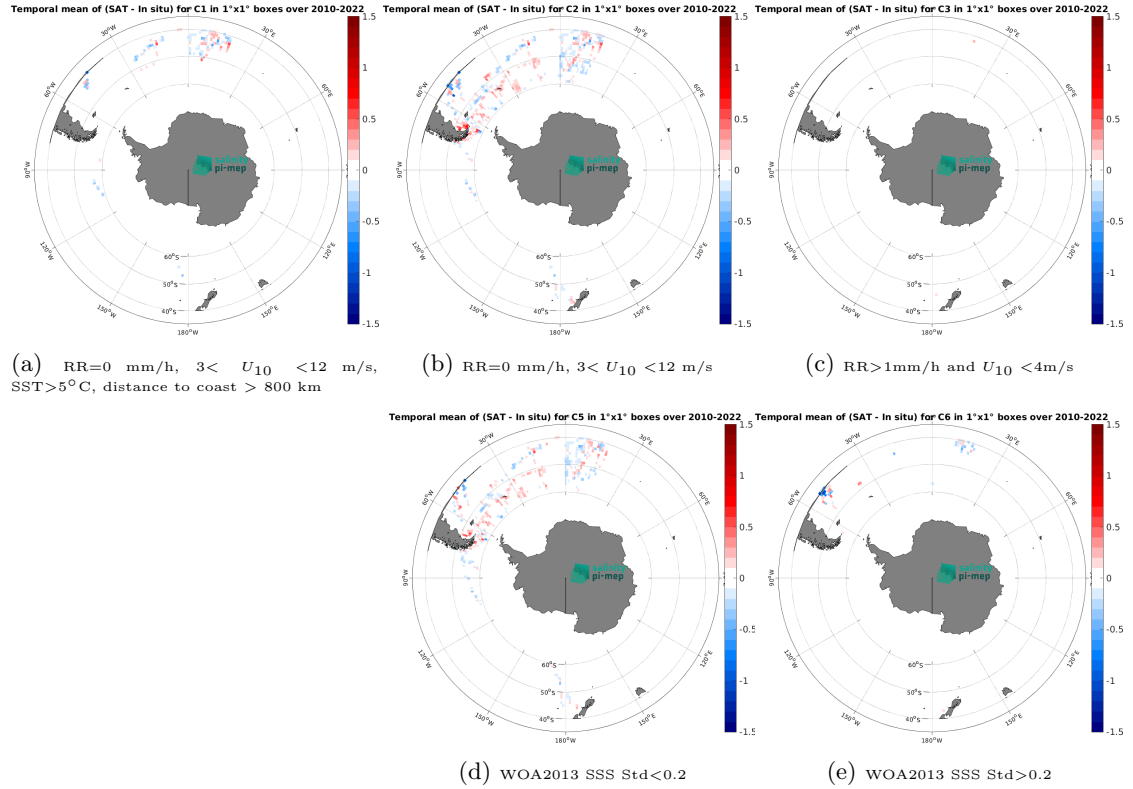
Figure 12: Temporal mean gridded over spatial boxes of size 1^{\circ}\times 1^{\circ} of \Delta\text{SSS} (SMOS SSS L3 v8 - 18 Days (CATDS-CEC-LOCEAN) - TSG (Polarstern)) for 5 different subdatasets corresponding to:RR=0 mm/h, 3 < U_{10} < 12 m/s, SST >5^{\circ}\text{C} , distance to coast > 800 km (a), RR=0 mm/h, 3 < U_{10} < 12 m/s (b), RR >1 mm/h and U_{10} < 4 m/s (c), WOA2013 SSS Std <0.2 (d), WOA2013 SSS Std >0.2 (e).
