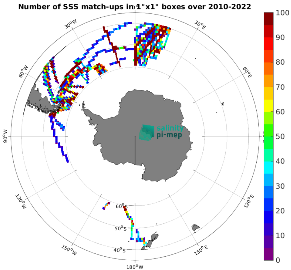
Figure 4: Number of SSS match-ups between TSG (Polarstern) SSS and the SMOS SSS L3 v8 - 18 Days (CATDS-CEC-LOCEAN) SSS product for the Roaring Forties and Furious Fifties Pi-MEP region over 1^\circ \times 1^\circ boxes and for the full satellite product period.
