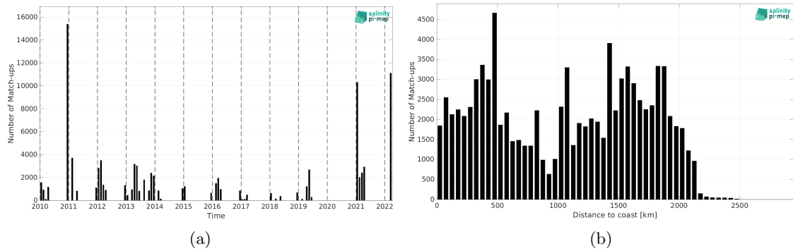
Figure 1: Number of match-ups between TSG (Polarstern) and SMOS SSS L3 v8 - 18 Days (CATDS-CEC-LOCEAN) SSS as a function of time (a) and as function of the distance to coast (b) over the Roaring Forties and Furious Fifties Pi-MEP region and for the full satellite product period.
