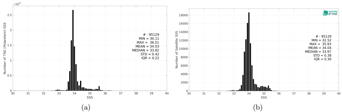
Figure 2: Histograms of SSS from TSG (Polarstern) (a) and SMOS SSS L3 v8 - 18 Days (CATDS-CEC-LOCEAN) (b) considering all match-up pairs per bins of 0.1 over the Roaring Forties and Furious Fifties Pi-MEP region and for the full satellite product period.
