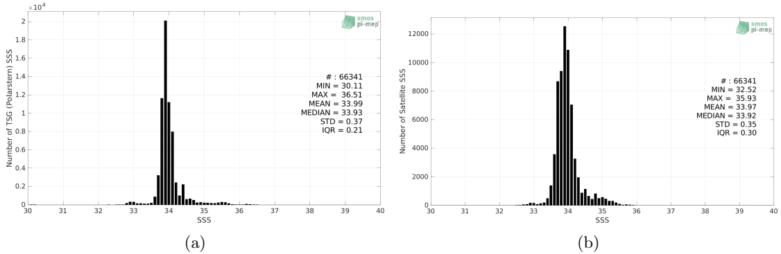
Figure 2: Histograms of SSS from TSG (Polarstern) (a) and SMOS SSS L3 v8 - 18 Days (CATDS-CECOS-LOCEAN) (b) considering all match-up pairs per bins of 0.1 over the Roaring Forties and Furious Fifties Pi-MEP region and for the full satellite product period.
