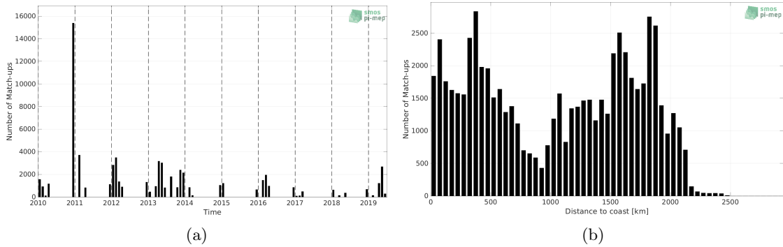
Figure 1: Number of match-ups between TSG (Polarstern) and SMOS SSS L3 v8 - 18 Days (CATDS-CECOS-LOCEAN) SSS as a function of time (a) and as function of the distance to coast (b) over the Roaring Forties and Furious Fifties Pi-MEP region and for the full satellite product period.
