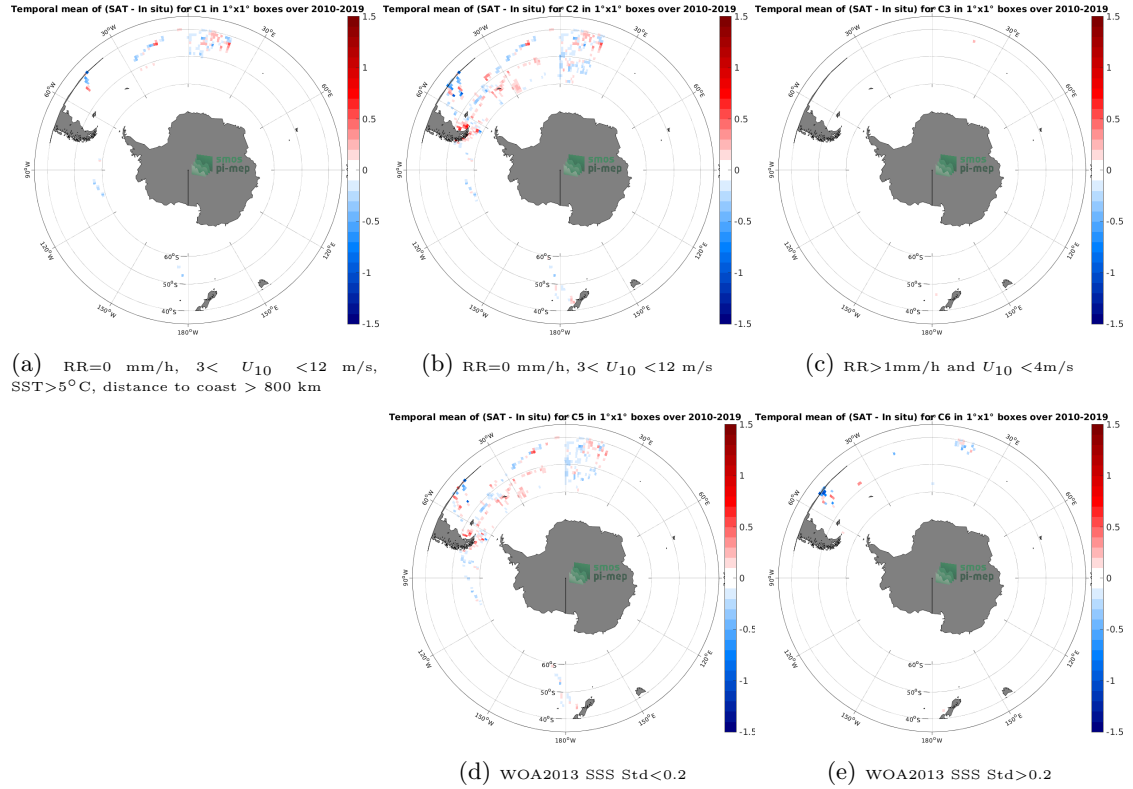
Figure 12: Temporal mean gridded over spatial boxes of size 1^{\circ}\times 1^{\circ} of \Delta\text{SSS} (SMOS SSS L3 v8 - 18 Days (CATDS-CECOS-LOCEAN) - TSG (Polarstern)) for 5 different subdatasets corresponding to:RR=0 mm/h, 3 < U_{10} < 12 m/s, SST >5^{\circ}\text{C} , distance to coast > 800 km (a), RR=0 mm/h, 3 < U_{10} < 12 m/s (b), RR >1 mm/h and U_{10} < 4 m/s (c), WOA2013 SSS Std <0.2 (d), WOA2013 SSS Std >0.2 (e).
