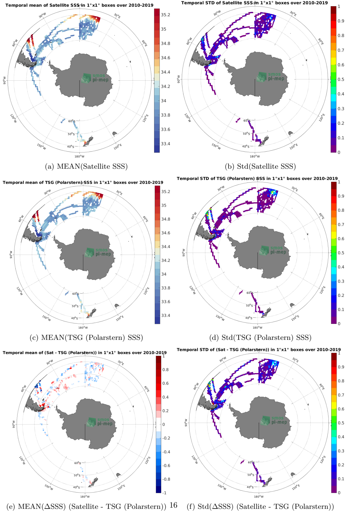
Figure 6: Temporal mean (left) and Std (right) of SSS from SMOS SSS L3 v8 - 18 Days (CATDS-CECOS-LOCEAN) (top), TSG (Polarstern) (middle), and of \Delta SSS (Satellite - TSG (Polarstern)). Only match-up pairs are used to generate these maps.
