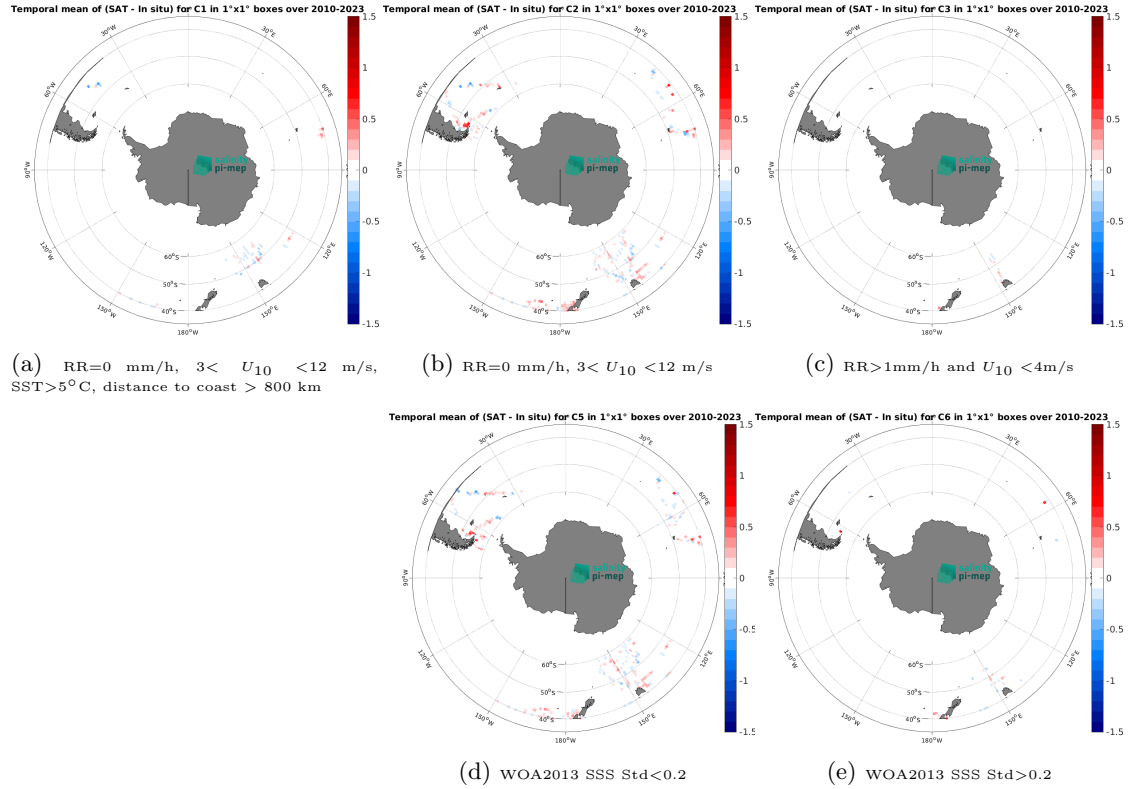
Figure 12: Temporal mean gridded over spatial boxes of size 1^{\circ}\times 1^{\circ} of \Delta\text{SSS} (SMOS SSS L3 v8 - 18 Days (CATDS-CEC-LOCEAN) - TSG (LEGOS-DM)) for 5 different subdatasets corresponding to:RR=0 mm/h, 3 < U_{10} < 12 m/s, SST >5^{\circ}\text{C} , distance to coast > 800 km (a), RR=0 mm/h, 3 < U_{10} < 12 m/s (b), RR >1 mm/h and U_{10} < 4 m/s (c), WOA2013 SSS Std <0.2 (d), WOA2013 SSS Std >0.2 (e).
