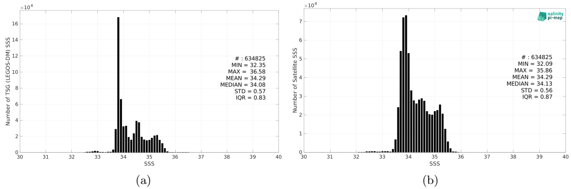
Figure 2: Histograms of SSS from TSG (LEGOS-DM) (a) and SMOS SSS L3 v8 - 18 Days (CATDS-CEC-LOCEAN) (b) considering all match-up pairs per bins of 0.1 over the Roaring Forties and Furious Fifties Pi-MEP region and for the full satellite product period.
