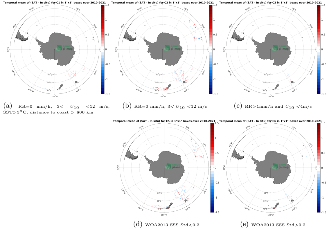
Figure 12: Temporal mean gridded over spatial boxes of size 1^{\circ}\times 1^{\circ} of \Delta\text{SSS} (SMOS SSS L3 v8 - 18 Days (CATDS-CECOS-LOCEAN) - TSG (LEGOS-DM)) for 5 different subdatasets corresponding to:RR=0 mm/h, 3 < U_{10} < 12 m/s, SST >5^{\circ}\text{C} , distance to coast > 800 km (a), RR=0 mm/h, 3 < U_{10} < 12 m/s (b), RR >1 mm/h and U_{10} < 4 m/s (c), WOA2013 SSS Std <0.2 (d), WOA2013 SSS Std >0.2 (e).
