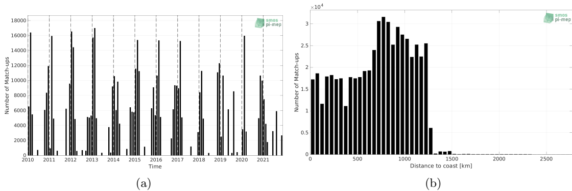
Figure 1: Number of match-ups between TSG (LEGOS-DM) and SMOS SSS L3 v8 - 18 Days (CATDS-CECOS-LOCEAN) SSS as a function of time (a) and as function of the distance to coast (b) over the Roaring Forties and Furious Fifties Pi-MEP region and for the full satellite product period.
