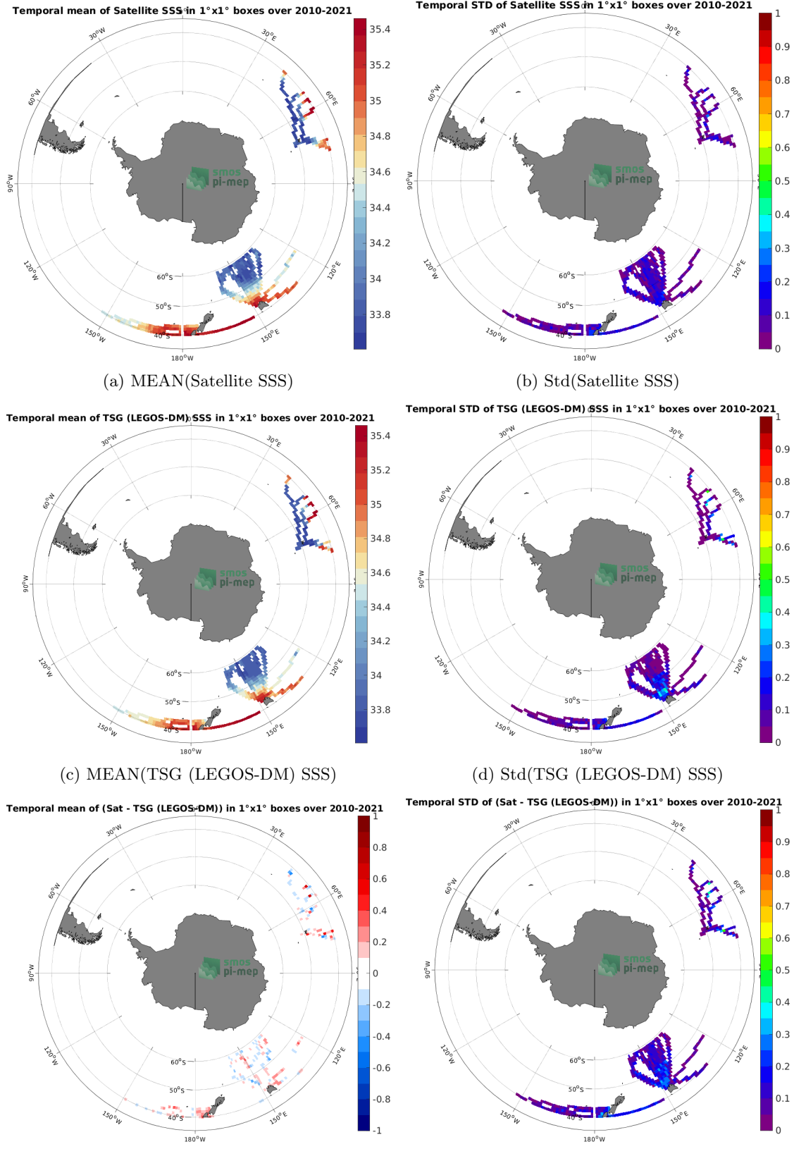
(e) MEAN( \Delta SSS) (Satellite - TSG (LEGOS-DM)) 16 (f) Std( \Delta SSS) (Satellite - TSG (LEGOS-DM)) Figure 6: Temporal mean (left) and Std (right) of SSS from SMOS SSS L3 v8 - 18 Days (CATDS-CECOS-LOCEAN) (top), TSG (LEGOS-DM) (middle), and of \Delta SSS (Satellite - TSG (LEGOS-DM)). Only match-up pairs are used to generate these maps.
