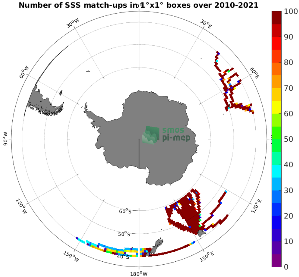
Figure 4: Number of SSS match-ups between TSG (LEGOS-DM) SSS and the SMOS SSS L3 v8 - 18 Days (CATDS-CECOS-LOCEAN) SSS product for the Roaring Forties and Furious Fifties Pi-MEP region over 1^\circ \times 1^\circ boxes and for the full satellite product period.
