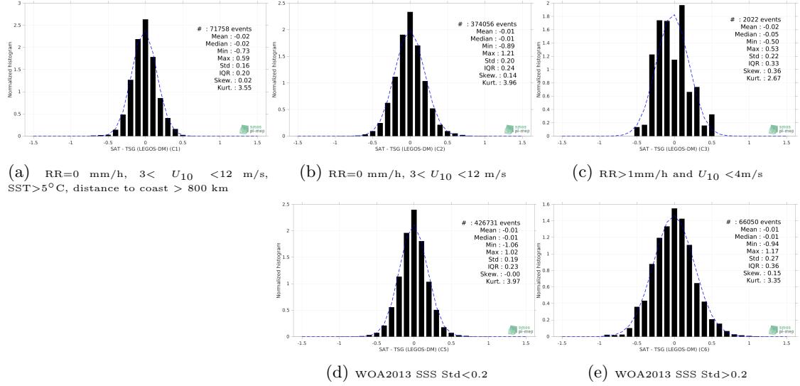
Figure 13: Normalized histogram of \Delta\text{SSS} (SMOS SSS L3 v8 - 18 Days (CATDS-CECOS-LOCEAN) - TSG (LEGOS-DM)) for 5 different subdatasets corresponding to: RR=0 mm/h, 3 < U_{10} < 12 m/s, SST>5°C, distance to coast > 800 km (a), RR=0 mm/h, 3 < U_{10} < 12 m/s (b), RR>1mm/h and U_{10} < 4 m/s (c), WOA2013 SSS Std<0.2 (d), WOA2013 SSS Std>0.2 (e).
