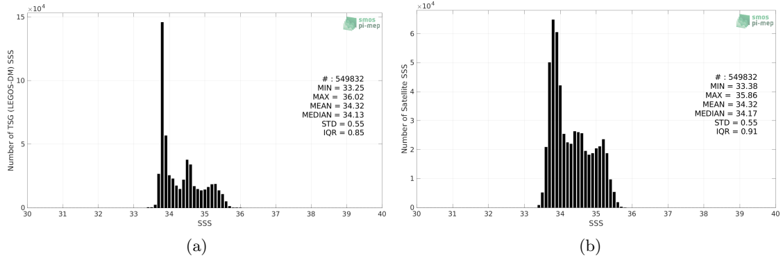
Figure 2: Histograms of SSS from TSG (LEGOS-DM) (a) and SMOS SSS L3 v8 - 18 Days (CATDS-CECOS-LOCEAN) (b) considering all match-up pairs per bins of 0.1 over the Roaring Forties and Furious Fifties Pi-MEP region and for the full satellite product period.
