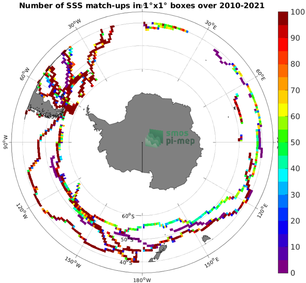
Figure 4: Number of SSS match-ups between TSG (GOSUD-Sailing-ship) SSS and the SMOS SSS L3 v8 - 18 Days (CATDS-CECOS-LOCEAN) SSS product for the Roaring Forties and Furious Fifties Pi-MEP region over 1^\circ \times 1^\circ boxes and for the full satellite product period.
