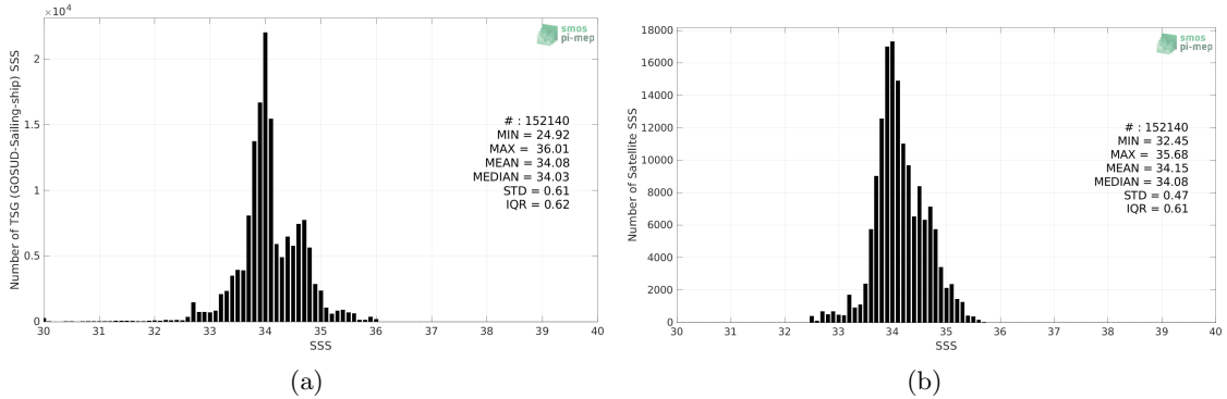
Figure 2: Histograms of SSS from TSG (GOSUD-Sailing-ship) (a) and SMOS SSS L3 v8 - 18 Days (CATDS-CECOS-LOCEAN) (b) considering all match-up pairs per bins of 0.1 over the Roaring Forties and Furious Fifties Pi-MEP region and for the full satellite product period.
