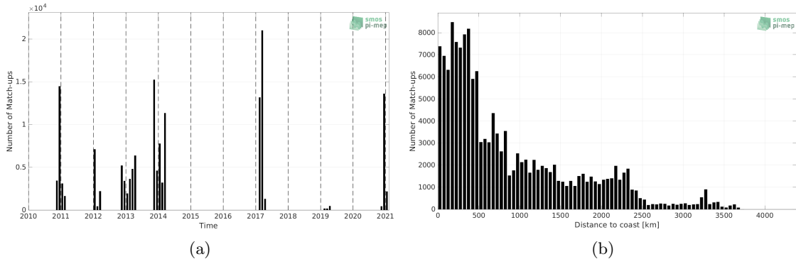
Figure 1: Number of match-ups between TSG (GOSUD-Sailing-ship) and SMOS SSS L3 v8 - 18 Days (CATDS-CECOS-LOCEAN) SSS as a function of time (a) and as function of the distance to coast (b) over the Roaring Forties and Furious Fifties Pi-MEP region and for the full satellite product period.
