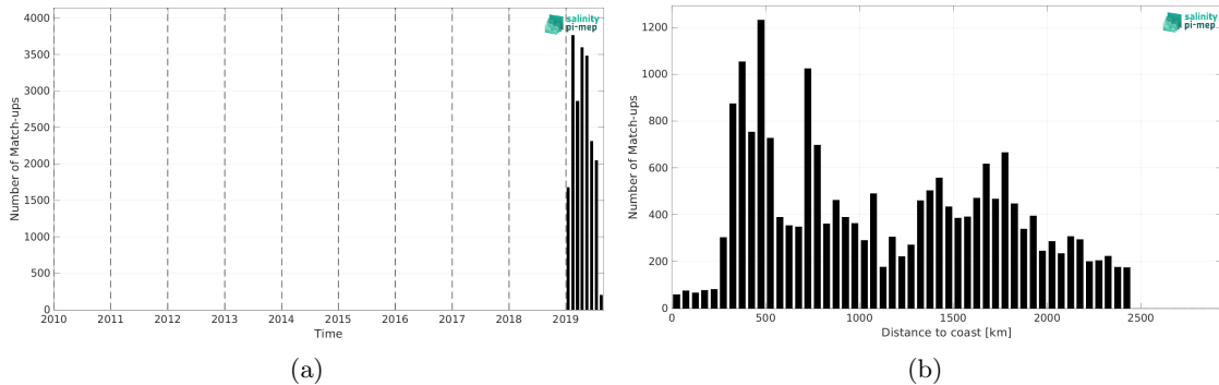
Figure 1: Number of match-ups between Saildrone and SMOS SSS L3 v8 - 18 Days (CATDS-CEC-LOCEAN) SSS as a function of time (a) and as function of the distance to coast (b) over the Roaring Forties and Furious Fifties Pi-MEP region and for the full satellite product period.
