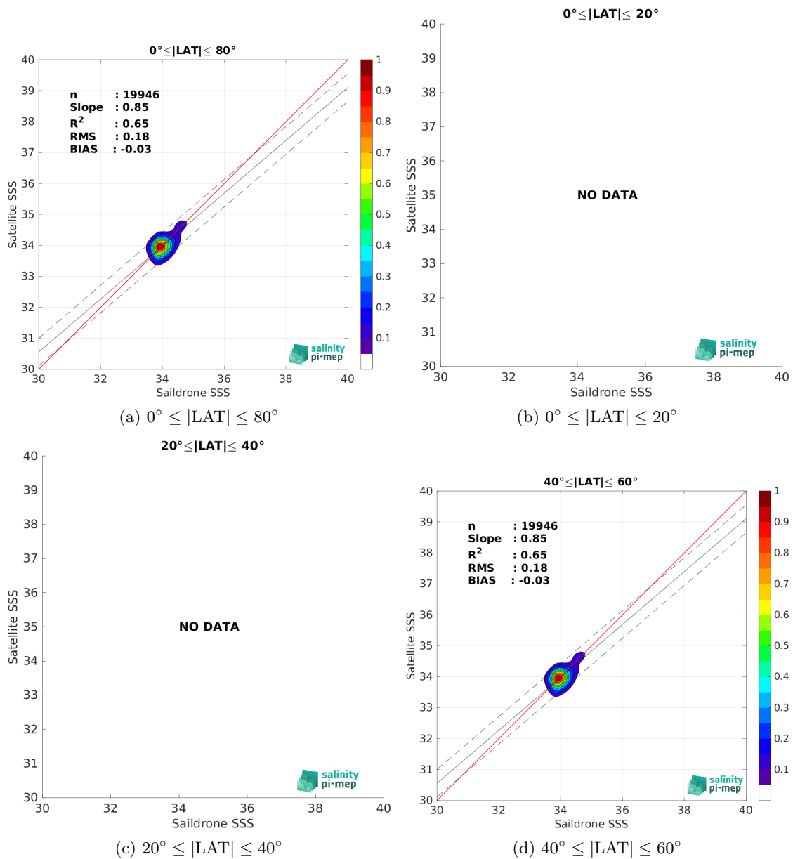
Figure 9: Contour maps of the concentration of SMOS SSS L3 v8 - 18 Days (CATDS-CEC-LOCEAN) SSS (y-axis) versus Sairdron SSS (x-axis) at match-up pairs for different latitude bands. For each plot, the red line shows x=y . The black thin and dashed lines indicate a linear fit through the data cloud and the \pm 95\% confidence levels, respectively. The number match-up pairs n , the slope and R^2 coefficient of the linear fit, the root mean square (RMS) and the mean bias between satellite and in situ data are indicated for each latitude band in each plots.
