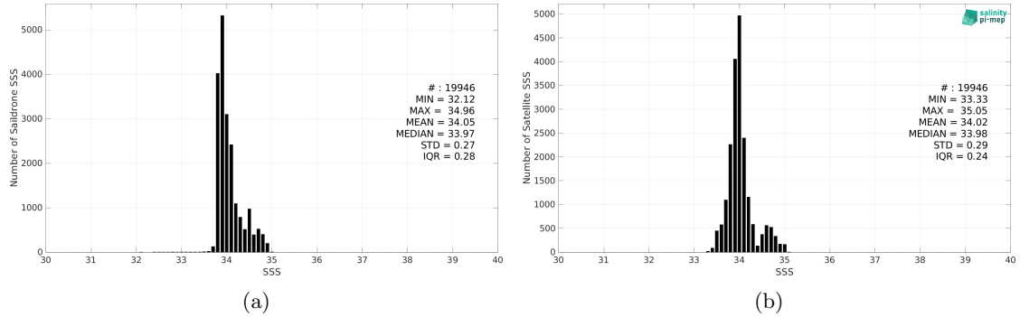
Figure 2: Histograms of SSS from Saildrone (a) and SMOS SSS L3 v8 - 18 Days (CATDS-CEC-LOCEAN) (b) considering all match-up pairs per bins of 0.1 over the Roaring Forties and Furious Fifties Pi-MEP region and for the full satellite product period.
