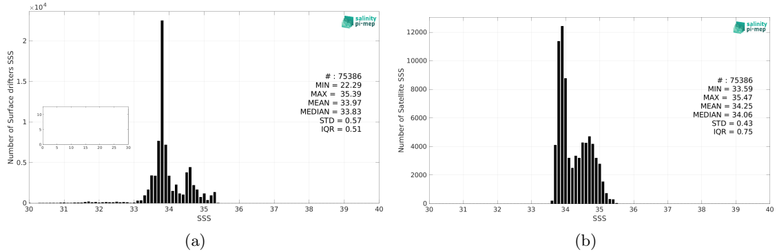
Figure 2: Histograms of SSS from Surface drifters (a) and SMOS SSS L3 v8 - 18 Days (CATDS-CEC-LOCEAN) (b) considering all match-up pairs per bins of 0.1 over the Roaring Forties and Furious Fifties Pi-MEP region and for the full satellite product period.
