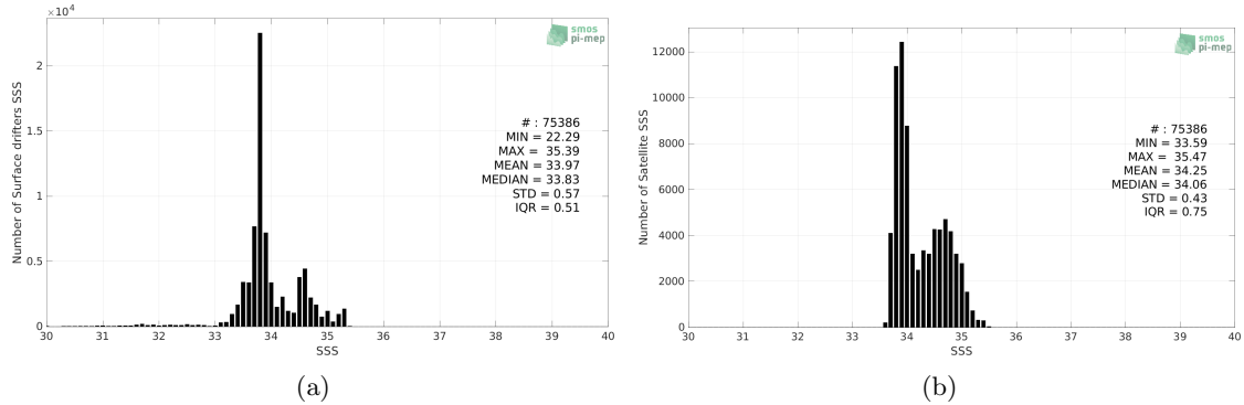
Figure 2: Histograms of SSS from Surface drifters (a) and SMOS SSS L3 v8 - 18 Days (CATDS-CECOS-LOCEAN) (b) considering all match-up pairs per bins of 0.1 over the Roaring Forties and Furious Fifties Pi-MEP region and for the full satellite product period.
