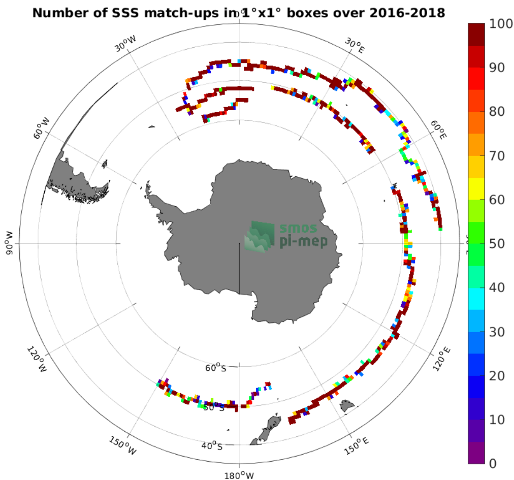
Figure 3: Number of SSS match-ups between Surface drifters SSS and the SMOS SSS L3 v8 - 18 Days (CATDS-CECOS-LOCEAN) SSS product for the Roaring Forties and Furious Fifties Pi-MEP region over 1^\circ \times 1^\circ boxes and for the full satellite product period.
