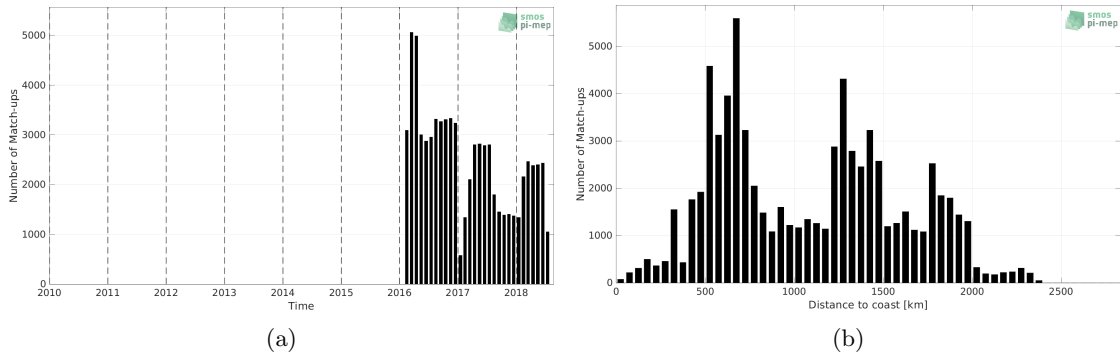
Figure 1: Number of match-ups between Surface drifters and SMOS SSS L3 v8 - 18 Days (CATDS-CECOS-LOCEAN) SSS as a function of time (a) and as function of the distance to coast (b) over the Roaring Forties and Furious Fifties Pi-MEP region and for the full satellite product period.
