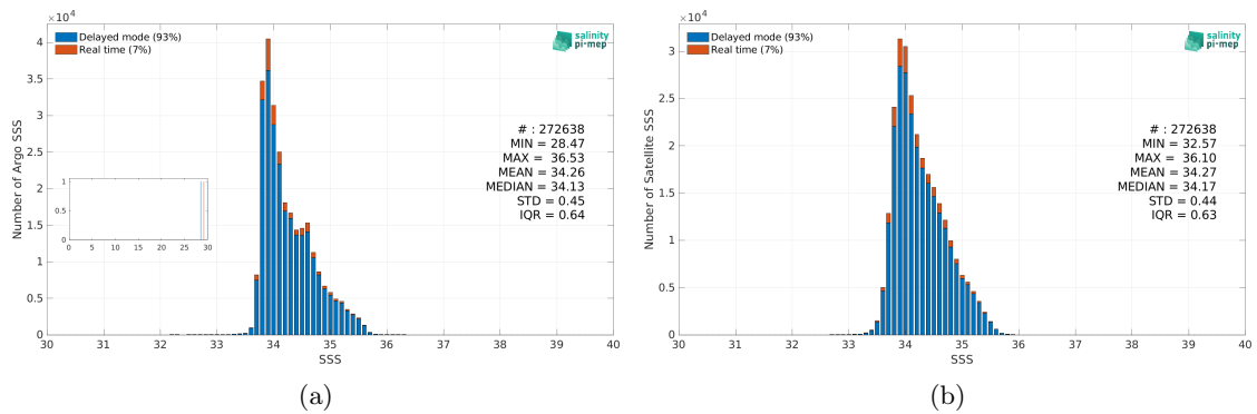
Figure 2: Histograms of SSS from Argo (a) and SMOS SSS L3 v8 - 18 Days (CATDS-CEC-LOCEAN) (b) considering all match-up pairs per bins of 0.1 over the Roaring Forties and Furious Fifties Pi-MEP region and for the full satellite product period.
