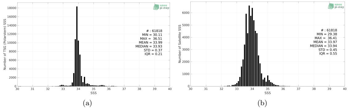
Figure 2: Histograms of SSS from TSG (Polarstern) (a) and SMOS SSS L3 v7 - 9 Days (CATDS-CECOS-LOCEAN) (b) considering all match-up pairs per bins of 0.1 over the Roaring Forties and Furious Fifties Pi-MEP region and for the full satellite product period.
