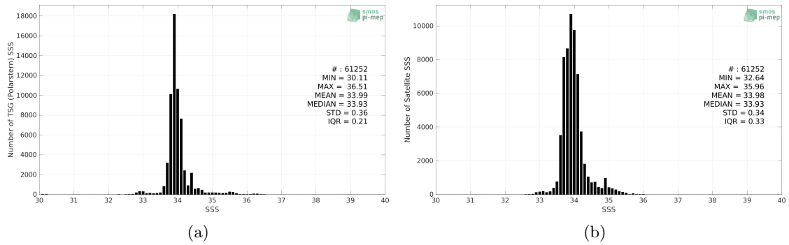
Figure 2: Histograms of SSS from TSG (Polarstern) (a) and SMOS SSS L3 v7 - 18 Days (CATDS-CECOS-LOCEAN) (b) considering all match-up pairs per bins of 0.1 over the Roaring Forties and Furious Fifties Pi-MEP region and for the full satellite product period.
