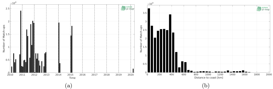
Figure 1: Number of match-ups between TSG (SAMOS) and SMOS SSS L3 v5 - 9 Days (CATDS-CECOS-LOCEAN) SSS as a function of time (a) and as function of the distance to coast (b) over the Roaring Forties and Furious Fifties Pi-MEP region and for the full satellite product period.
