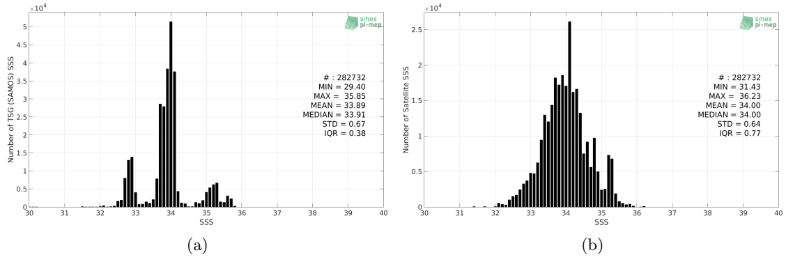
Figure 2: Histograms of SSS from TSG (SAMOS) (a) and SMOS SSS L3 v5 - 9 Days (CATDS-CECOS-LOCEAN) (b) considering all match-up pairs per bins of 0.1 over the Roaring Forties and Furious Fifties Pi-MEP region and for the full satellite product period.
