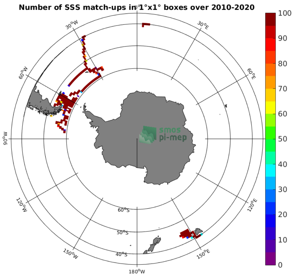
Figure 4: Number of SSS match-ups between TSG (SAMOS) SSS and the SMOS SSS L3 v5 - 9 Days (CATDS-CECOS-LOCEAN) SSS product for the Roaring Forties and Furious Fifties Pi-MEP region over 1^\circ \times 1^\circ boxes and for the full satellite product period.
