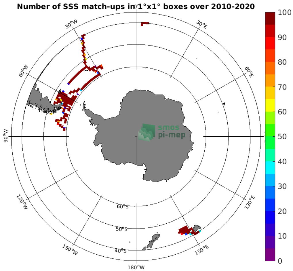
Figure 4: Number of SSS match-ups between TSG (SAMOS) SSS and the SMOS SSS L3 v5 - 9 Days (CATDS-CECOS-LOCEAN) SSS product for the Roaring Forties and Furious Fifties Pi-MEP region over 1^\circ \times 1^\circ boxes and for the full satellite product period.
