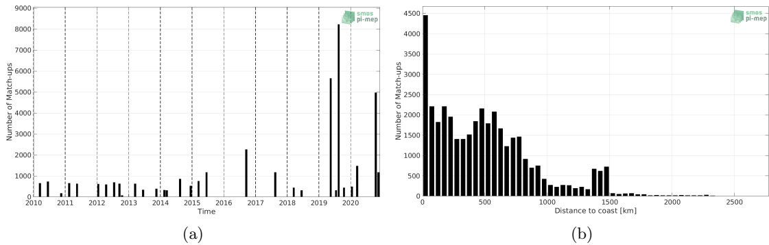
Figure 1: Number of match-ups between TSG (LEGOS-DM) and SMOS SSS L3 v5 - 9 Days (CATDS-CECOS-LOCEAN) SSS as a function of time (a) and as function of the distance to coast (b) over the Roaring Forties and Furious Fifties Pi-MEP region and for the full satellite product period.
