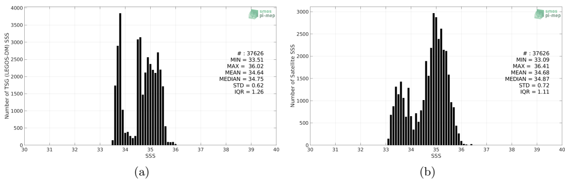
Figure 2: Histograms of SSS from TSG (LEGOS-DM) (a) and SMOS SSS L3 v5 - 9 Days (CATDS-CECOS-LOCEAN) (b) considering all match-up pairs per bins of 0.1 over the Roaring Forties and Furious Fifties Pi-MEP region and for the full satellite product period.
