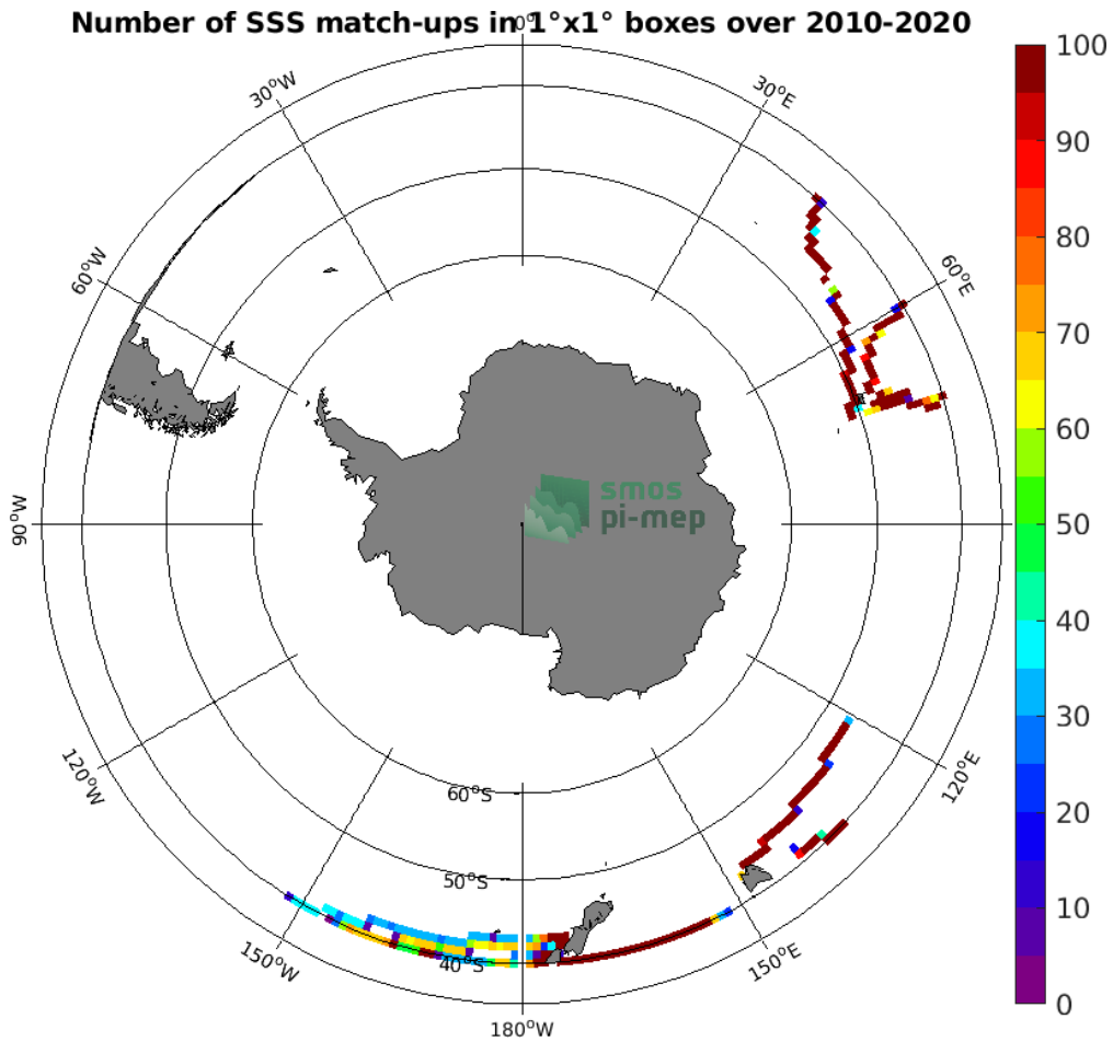
Figure 4: Number of SSS match-ups between TSG (LEGOS-DM) SSS and the SMOS SSS L3 v5 - 9 Days (CATDS-CECOS-LOCEAN) SSS product for the Roaring Forties and Furious Fifties Pi-MEP region over 1^\circ \times 1^\circ boxes and for the full satellite product period.
