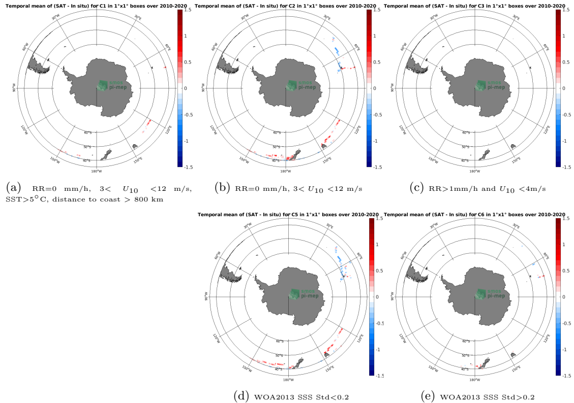
Figure 12: Temporal mean gridded over spatial boxes of size 1^{\circ}\times 1^{\circ} of \Delta\text{SSS} (SMOS SSS L3 v5 - 9 Days (CATDS-CECOS-LOCEAN) - TSG (LEGOS-DM)) for 5 different subdatasets corresponding to:RR=0 mm/h, 3 < U_{10} < 12 m/s, SST >5^{\circ}\text{C} , distance to coast > 800 km (a), RR=0 mm/h, 3 < U_{10} < 12 m/s (b), RR >1 mm/h and U_{10} < 4 m/s (c), WOA2013 SSS Std <0.2 (d), WOA2013 SSS Std >0.2 (e).
