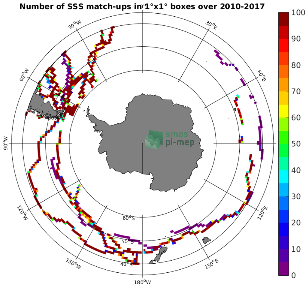
Figure 4: Number of SSS match-ups between TSG (GOSUD-Sailing-ship) SSS and the SMOS SSS L3 v5 - 9 Days (CATDS-CECOS-LOCEAN) SSS product for the Roaring Forties and Furious Fifties Pi-MEP region over 1^\circ \times 1^\circ boxes and for the full satellite product period.
