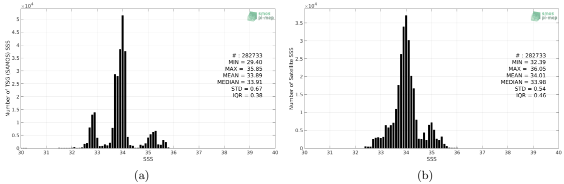
Figure 2: Histograms of SSS from TSG (SAMOS) (a) and SMOS SSS L3 v5 - 18 Days (CATDS-CECOS-LOCEAN) (b) considering all match-up pairs per bins of 0.1 over the Roaring Forties and Furious Fifties Pi-MEP region and for the full satellite product period.
