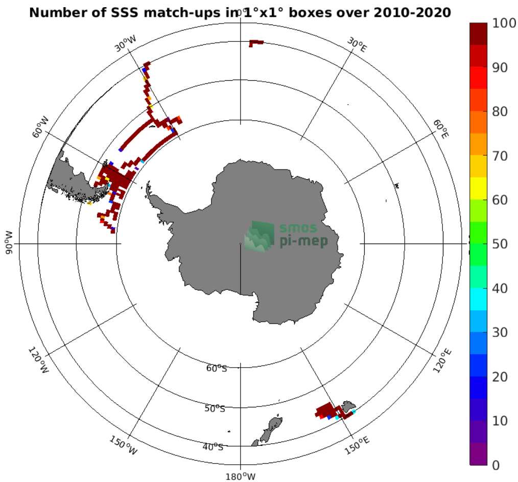
Figure 4: Number of SSS match-ups between TSG (SAMOS) SSS and the SMOS SSS L3 v5 - 18 Days (CATDS-CECOS-LOCEAN) SSS product for the Roaring Forties and Furious Fifties Pi-MEP region over 1°x1° boxes and for the full satellite product period.
