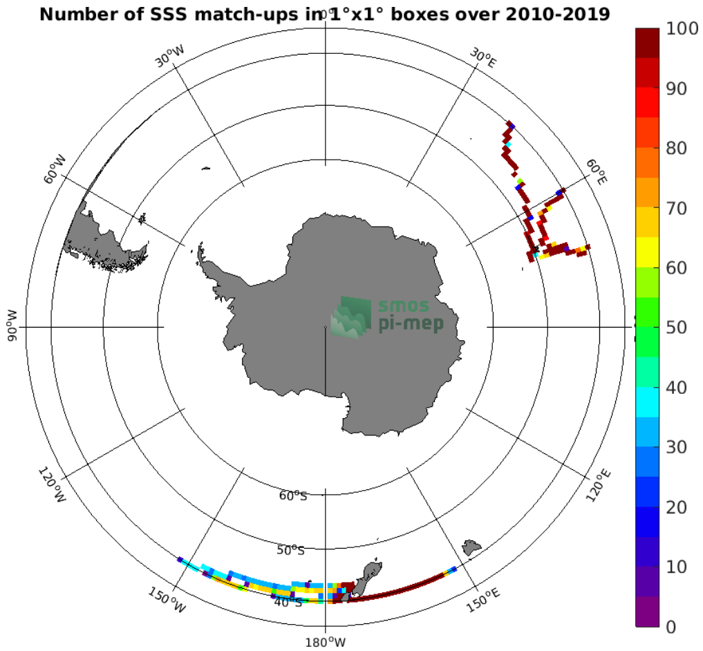
Figure 4: Number of SSS match-ups between TSG (LEGOS-DM) SSS and the SMOS SSS L3 v5 - 18 Days (CATDS-CECOS-LOCEAN) SSS product for the Roaring Forties and Furious Fifties Pi-MEP region over 1^\circ \times 1^\circ boxes and for the full satellite product period.
