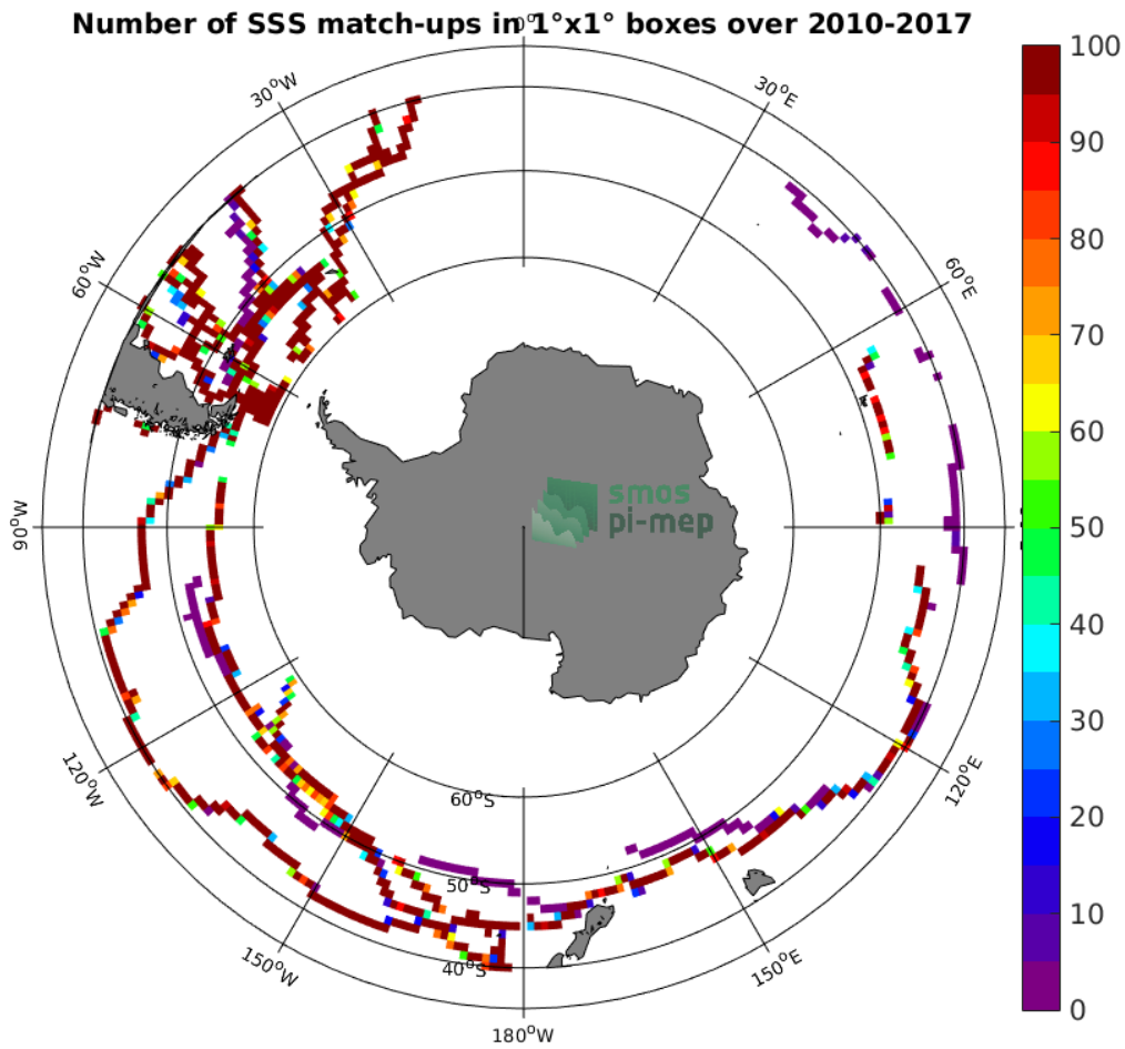
Figure 4: Number of SSS match-ups between TSG (GOSUD-Sailing-ship) SSS and the SMOS SSS L3 v5 - 18 Days (CATDS-CECOS-LOCEAN) SSS product for the Roaring Forties and Furious Fifties Pi-MEP region over 1^\circ \times 1^\circ boxes and for the full satellite product period.
