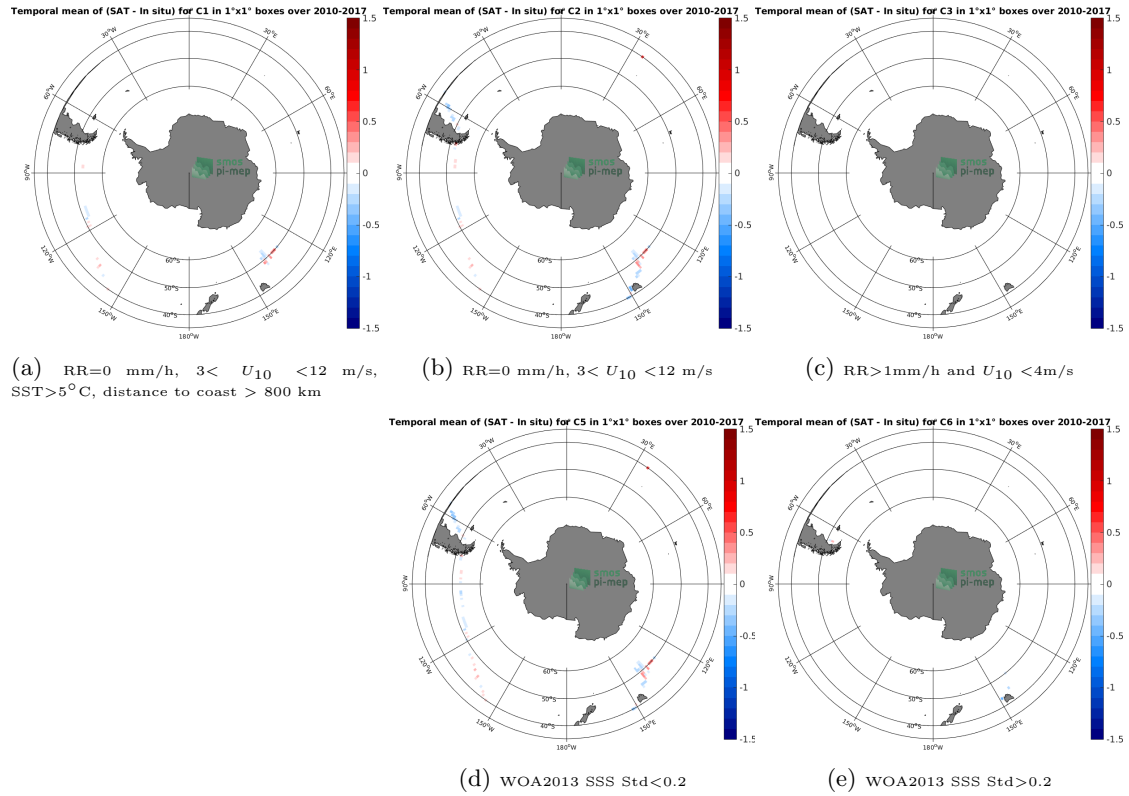
Figure 12: Temporal mean gridded over spatial boxes of size 1^\circ \times 1^\circ of \Delta SSS (SMOS SSS L3 v5 - 18 Days (CATDS-CECOS-LOCEAN) - TSG (GOSUD-Research-vessel)) for 5 different sub-datasets corresponding to: RR=0 mm/h, 3 < U_{10} < 12 m/s, SST>5°C, distance to coast > 800 km (a), RR=0 mm/h, 3 < U_{10} < 12 m/s (b), RR>1mm/h and U_{10} < 4 m/s (c), WOA2013 SSS Std<0.2 (d), WOA2013 SSS Std>0.2 (e).
