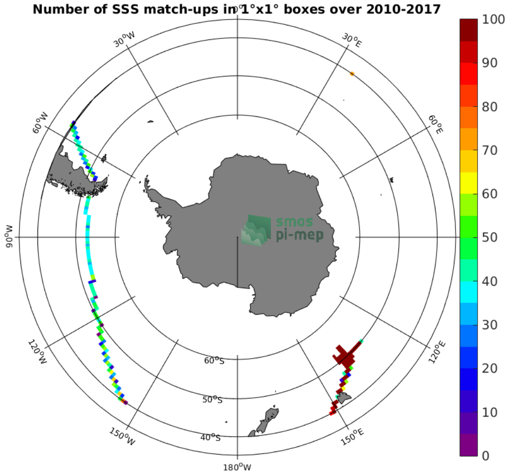
Figure 4: Number of SSS match-ups between TSG (GOSUD-Research-vessel) SSS and the SMOS SSS L3 v5 - 18 Days (CATDS-CECOS-LOCEAN) SSS product for the Roaring Forties and Furious Fifties Pi-MEP region over 1^\circ \times 1^\circ boxes and for the full satellite product period.
