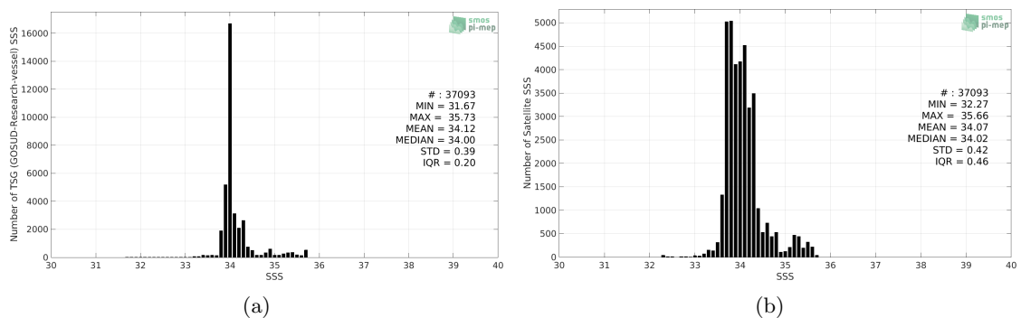
Figure 2: Histograms of SSS from TSG (GOSUD-Research-vessel) (a) and SMOS SSS L3 v5 - 18 Days (CATDS-CECOS-LOCEAN) (b) considering all match-up pairs per bins of 0.1 over the Roaring Forties and Furious Fifties Pi-MEP region and for the full satellite product period.
