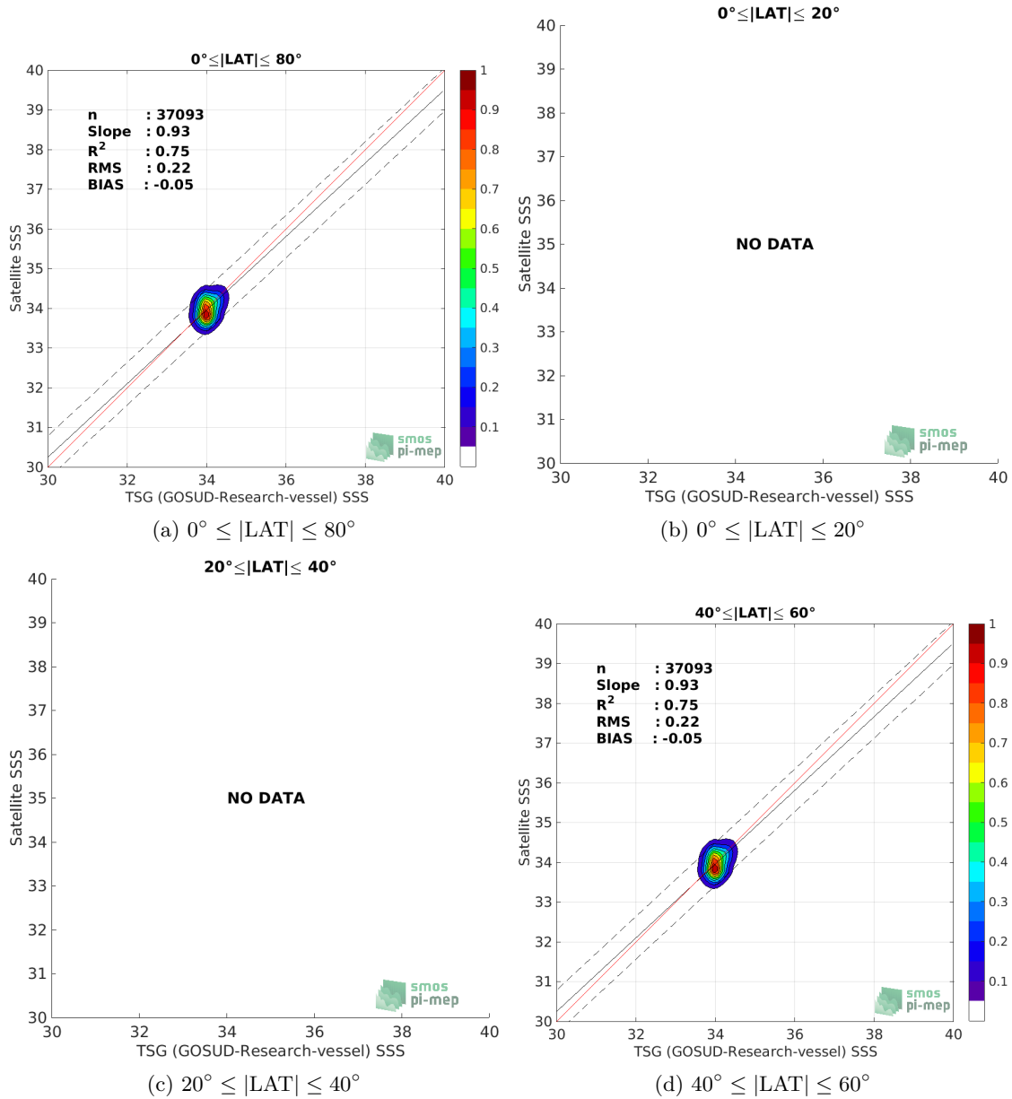
Figure 9: Contour maps of the concentration of SMOS SSS L3 v5 - 18 Days (CATDS-CECOS-LOCEAN) SSS ( y -axis) versus TSG (GOSUD-Research-vessel) SSS ( x -axis) at match-up pairs for different latitude bands. For each plot, the red line shows x=y . The black thin and dashed lines indicate a linear fit through the data cloud and the \pm 95\% confidence levels, respectively. The number match-up pairs n , the slope and R^2 coefficient of the linear fit, the root mean square (RMS) and the mean bias between satellite and in situ data are indicated for each latitude band in each plots.
