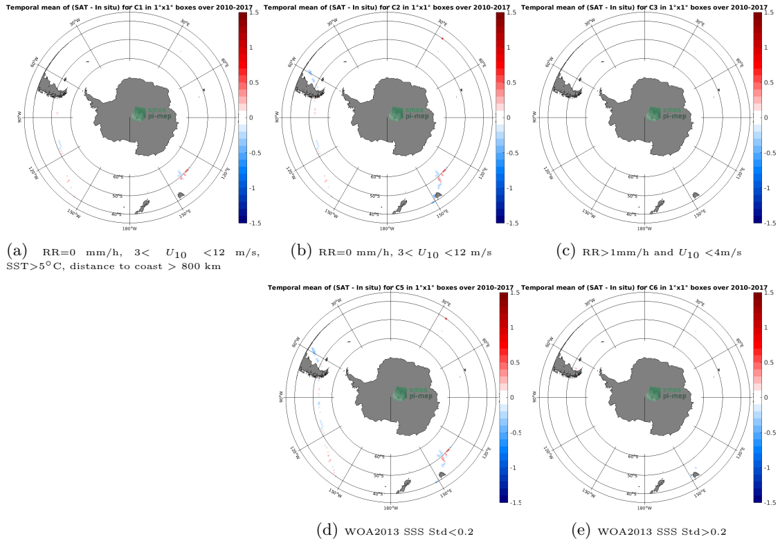
Figure 12: Temporal mean gridded over spatial boxes of size 1°x1° of \Delta SSS (SMOS SSS L3 v5 - 18 Days (CATDS-CECOS-LOCEAN) - TSG (GOSUD-Research-vessel)) for 5 different subdatasets corresponding to:RR=0 mm/h, 3 < U_{10} < 12 m/s, SST>5°C, distance to coast > 800 km (a), RR=0 mm/h, 3 < U_{10} < 12 m/s (b), RR>1mm/h and U_{10} < 4 m/s (c), WOA2013 SSS Std<0.2 (d), WOA2013 SSS Std>0.2 (e).
