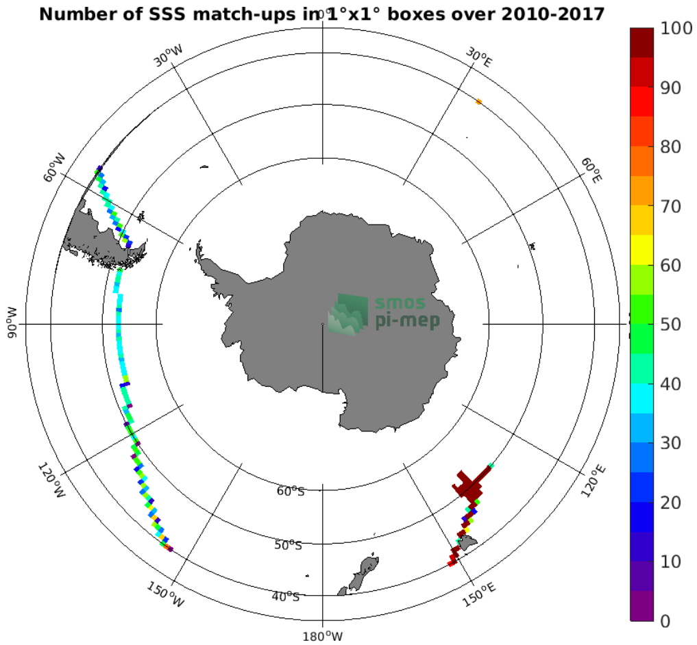
Figure 4: Number of SSS match-ups between TSG (GOSUD-Research-vessel) SSS and the SMOS SSS L3 v5 - 18 Days (CATDS-CECOS-LOCEAN) SSS product for the Roaring Forties and Furious Fifties Pi-MEP region over 1°x1° boxes and for the full satellite product period.
