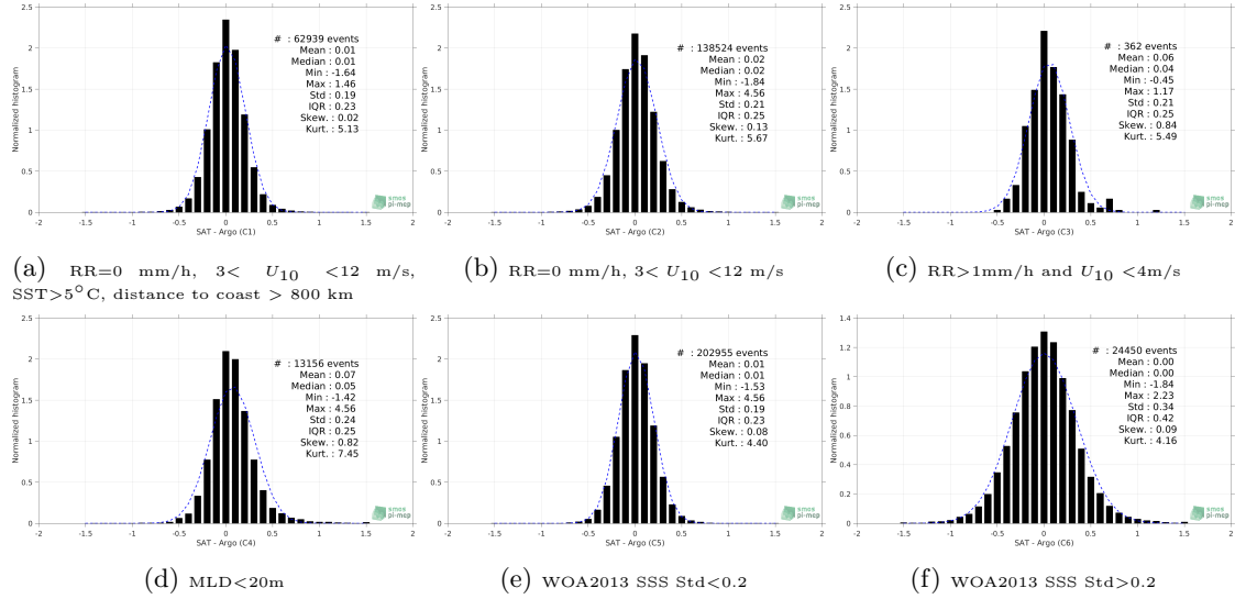
Figure 13: Normalized histogram of \Delta SSS (SMOS SSS L3 v5 - 18 Days (CATDS-CECOS-LOCEAN) - Argo) for 6 different subdatasets corresponding to: RR=0 mm/h, 3 < U_{10} < 12 m/s, SST > 5°C, distance to coast > 800 km (a), RR=0 mm/h, 3 < U_{10} < 12 m/s (b), RR > 1mm/h and U_{10} < 4 m/s (c), MLD < 20m (d), WOA2013 SSS Std < 0.2 (e), WOA2013 SSS Std > 0.2 (f).
