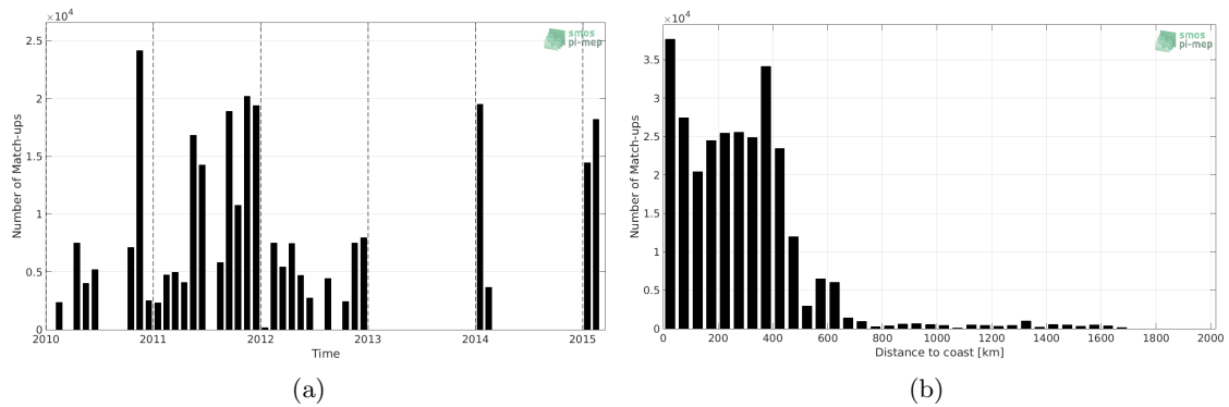
Figure 1: Number of match-ups between TSG (SAMOS) and SMOS SSS L3 v4 - 9 Days (CATDS-CECOS-LOCEAN) SSS as a function of time (a) and as function of the distance to coast (b) over the Roaring Forties and Furious Fifties Pi-MEP region and for the full satellite product period.
