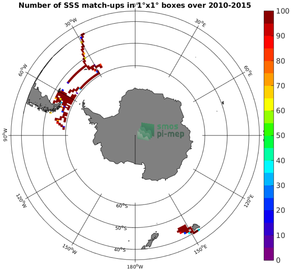
Figure 4: Number of SSS match-ups between TSG (SAMOS) SSS and the SMOS SSS L3 v4 - 9 Days (CATDS-CECOS-LOCEAN) SSS product for the Roaring Forties and Furious Fifties Pi-MEP region over 1^\circ \times 1^\circ boxes and for the full satellite product period.
