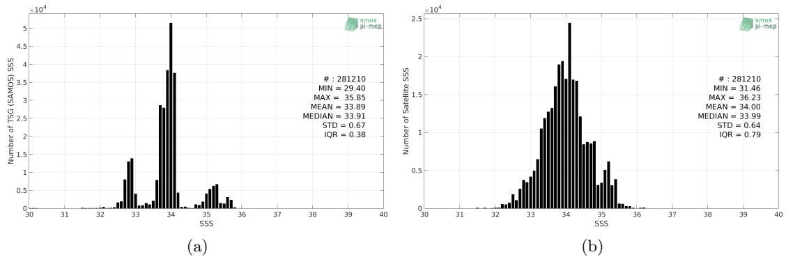
Figure 2: Histograms of SSS from TSG (SAMOS) (a) and SMOS SSS L3 v4 - 9 Days (CATDS-CECOS-LOCEAN) (b) considering all match-up pairs per bins of 0.1 over the Roaring Forties and Furious Fifties Pi-MEP region and for the full satellite product period.
