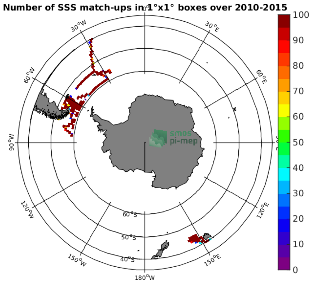
Figure 4: Number of SSS match-ups between TSG-SAMOS SSS and the SMOS-L3-CATDS-CECOS-LOCEAN-V4-9DAYS-25KM SSS product for the Roaring Forties and Furious Fifties Pi-MEP region over 1^\circ \times 1^\circ boxes and for the full satellite product period.
