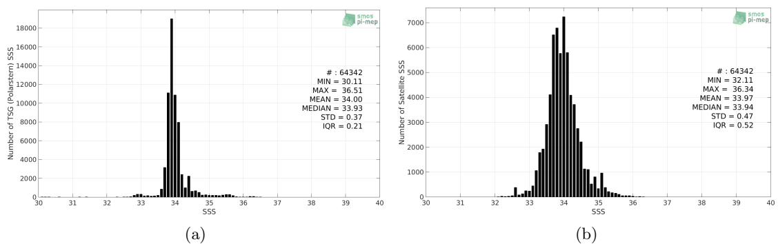
Figure 2: Histograms of SSS from TSG (Polarstern) (a) and SMOS SSS L3 v4 - 9 Days (CATDS-CECOS-LOCEAN) (b) considering all match-up pairs per bins of 0.1 over the Roaring Forties and Furious Fifties Pi-MEP region and for the full satellite product period.
