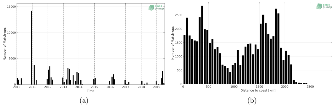
Figure 1: Number of match-ups between TSG (Polarstern) and SMOS SSS L3 v4 - 9 Days (CATDS-CECOS-LOCEAN) SSS as a function of time (a) and as function of the distance to coast (b) over the Roaring Forties and Furious Fifties Pi-MEP region and for the full satellite product period.
