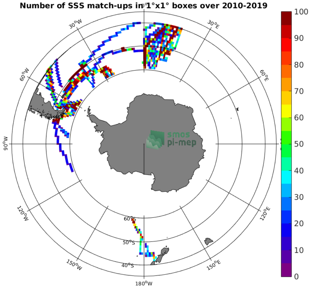
Figure 4: Number of SSS match-ups between TSG (Polarstern) SSS and the SMOS SSS L3 v4 - 9 Days (CATDS-CECOS-LOCEAN) SSS product for the Roaring Forties and Furious Fifties Pi-MEP region over 1^\circ \times 1^\circ boxes and for the full satellite product period.
